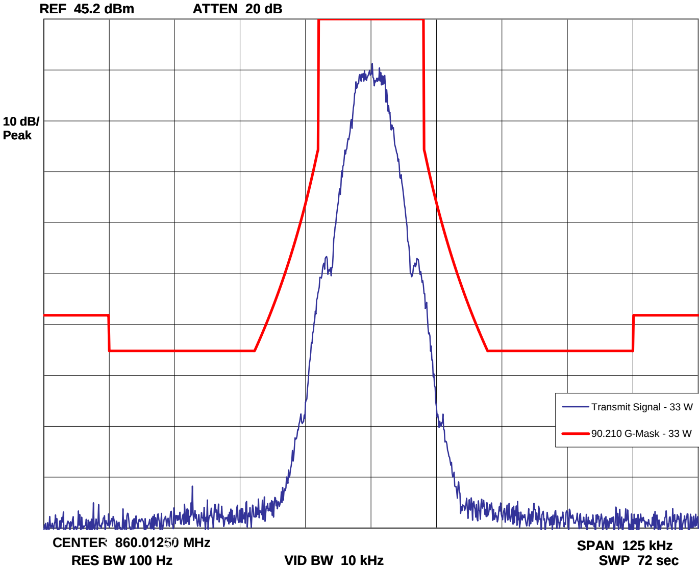
Occupied Bandwidth -- Four-Level Widepulse Astro - 33 Watts
