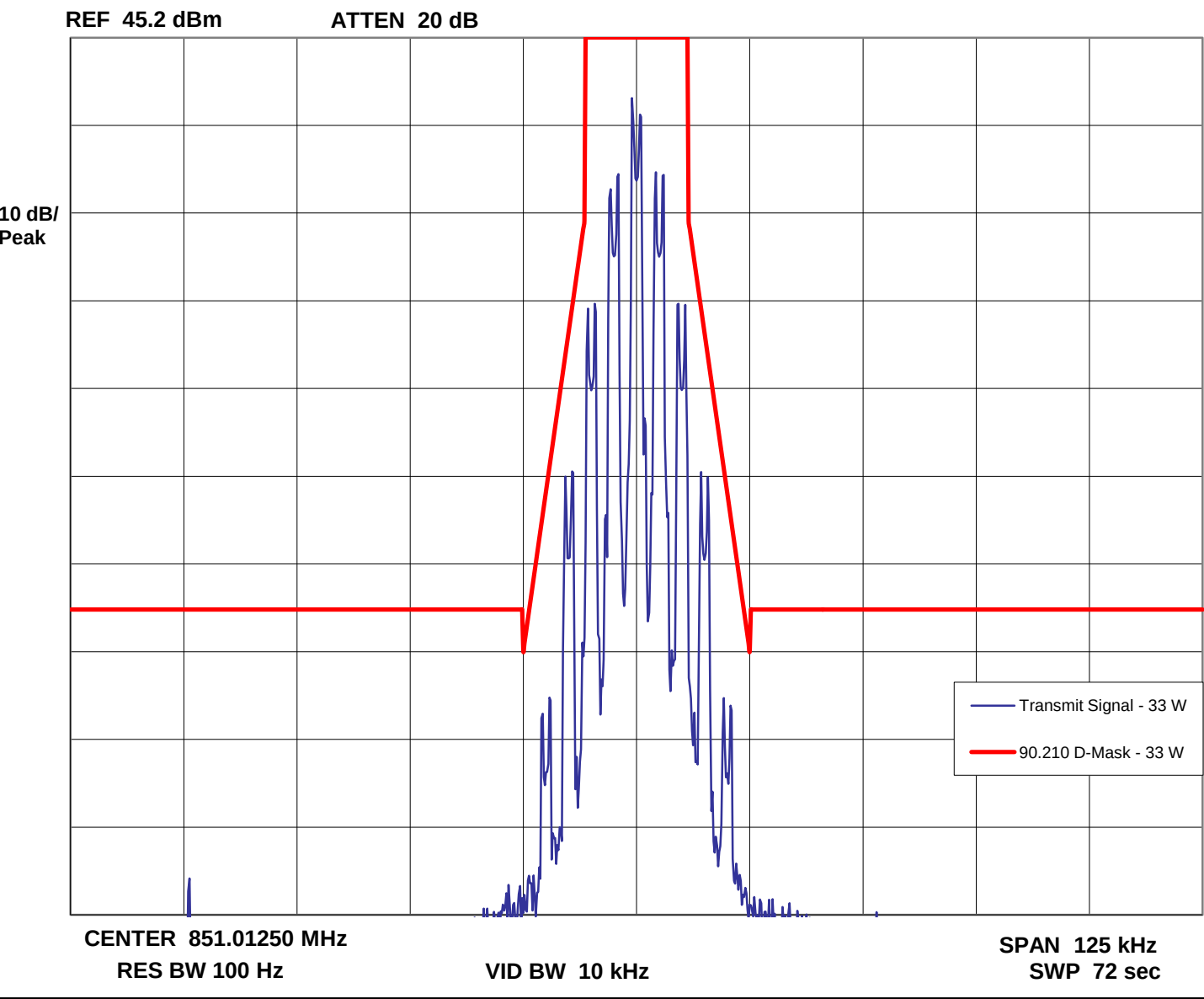
Occupied Bandwidth - 12.5 kHz Channels - Carrier with 2500 Hz Audio and 627 DPL
