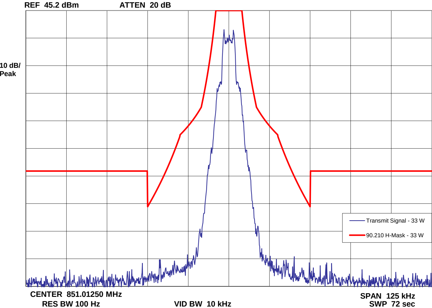
Occupied Bandwidth -- Trunking Control Data - 3600 bps FSK Modulation - 33 Watts
