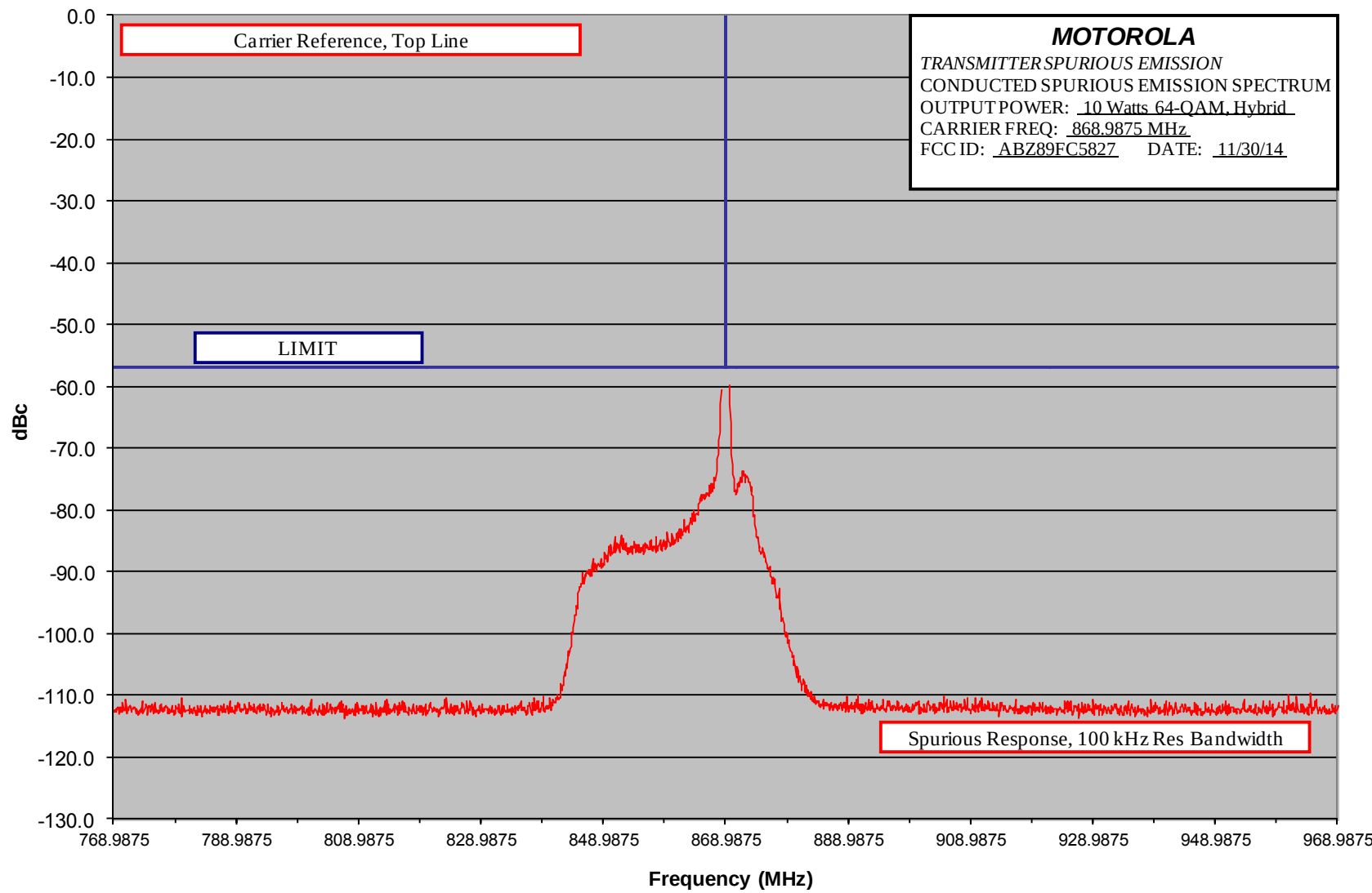
MTS 2 Conducted Spurious Emission Spectrum – 10 Watts 64-QAM – 200 MHz Span – High End of Band
