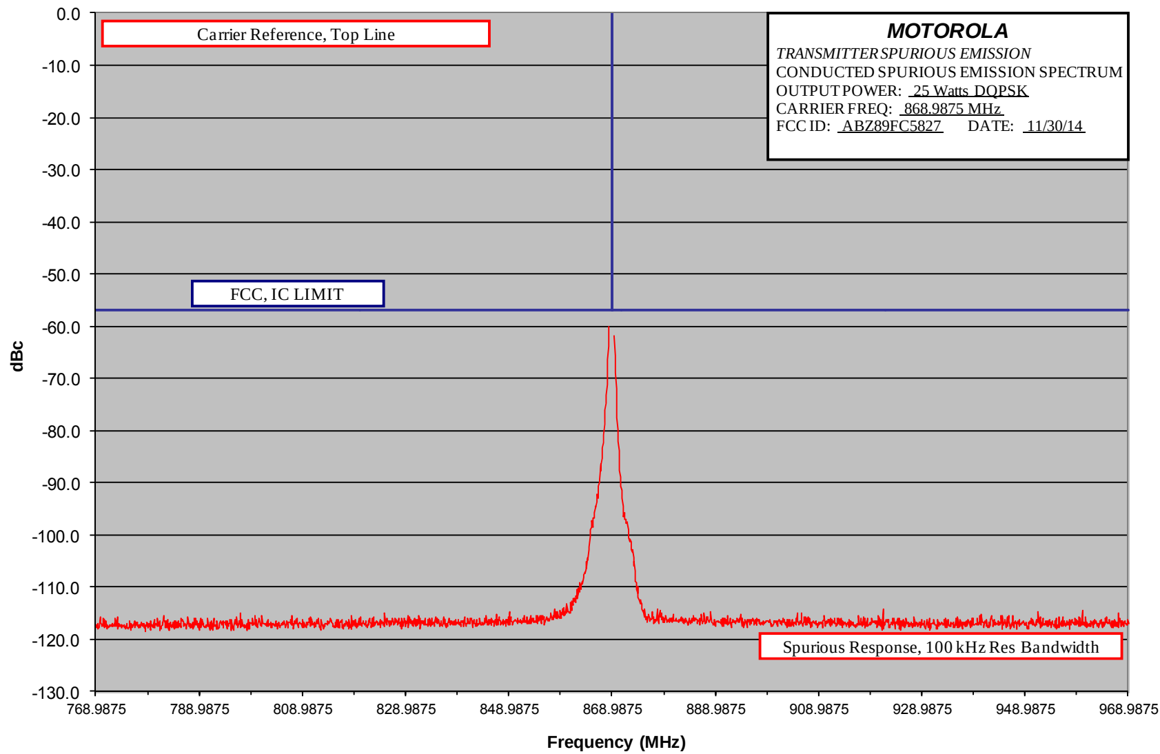
MTS 4 Conducted Spurious Emission Spectrum – 25 Watts DQPSK – 200 MHz Span – High End of Band
