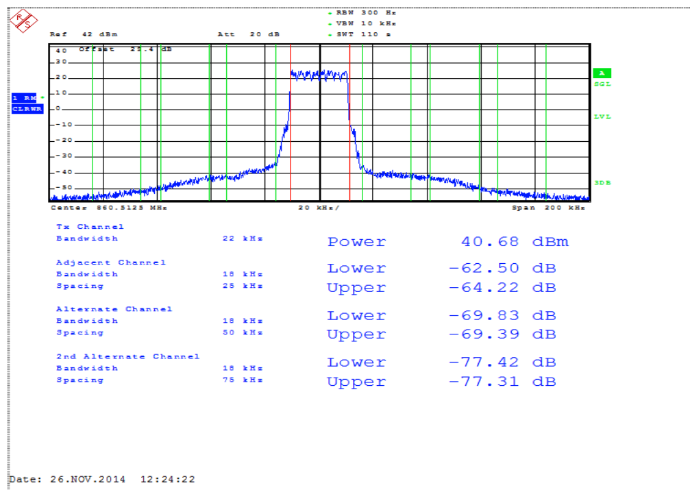
64-QAM, 860.5125 MHz, 10 Watts (Average) – MTS 2
