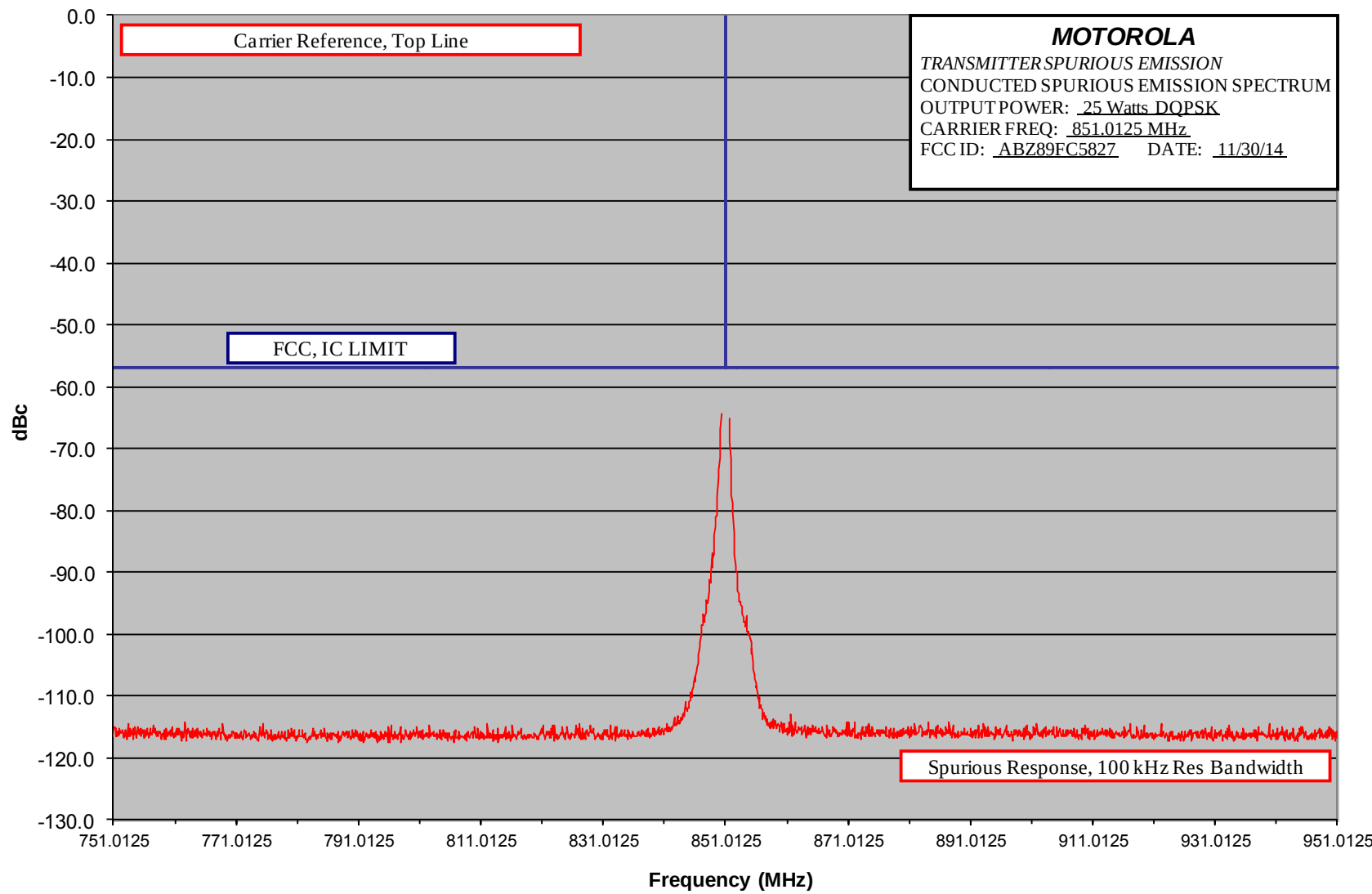
MTS 4 Conducted Spurious Emission Spectrum – 25 Watts DQPSK – 200 MHz Span – Low End of Band
