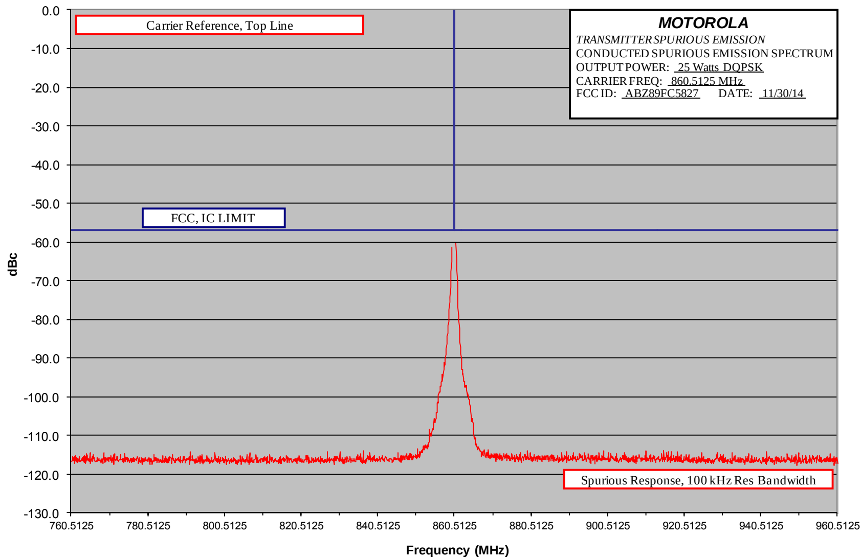
MTS 4 Conducted Spurious Emission Spectrum – 25 Watts DQPSK – 200 MHz Span – Middle of Band
