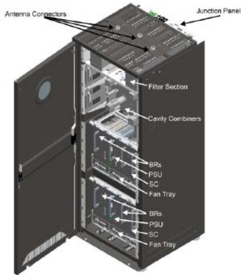
MTS 4 Base Radio Cabinet
