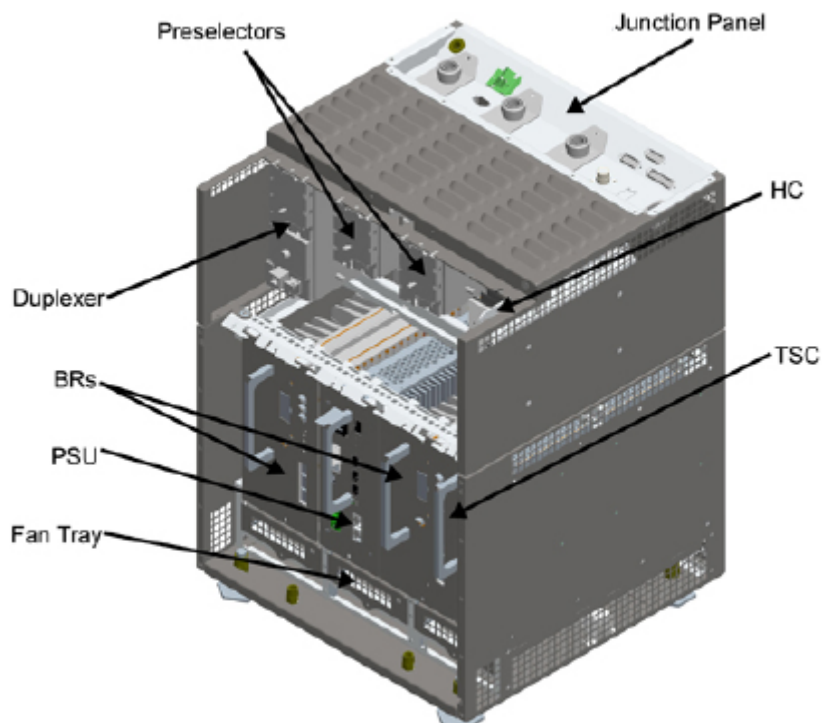
MTS 2 Base Radio Cabinet
