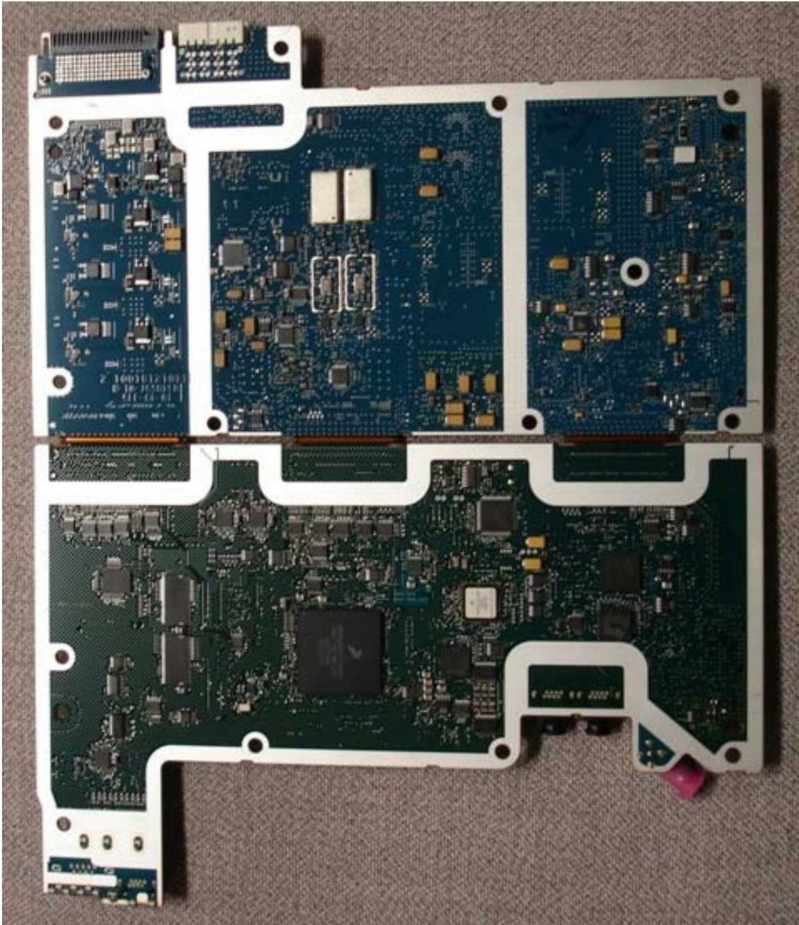
Internal Back View – Transceiver Module
