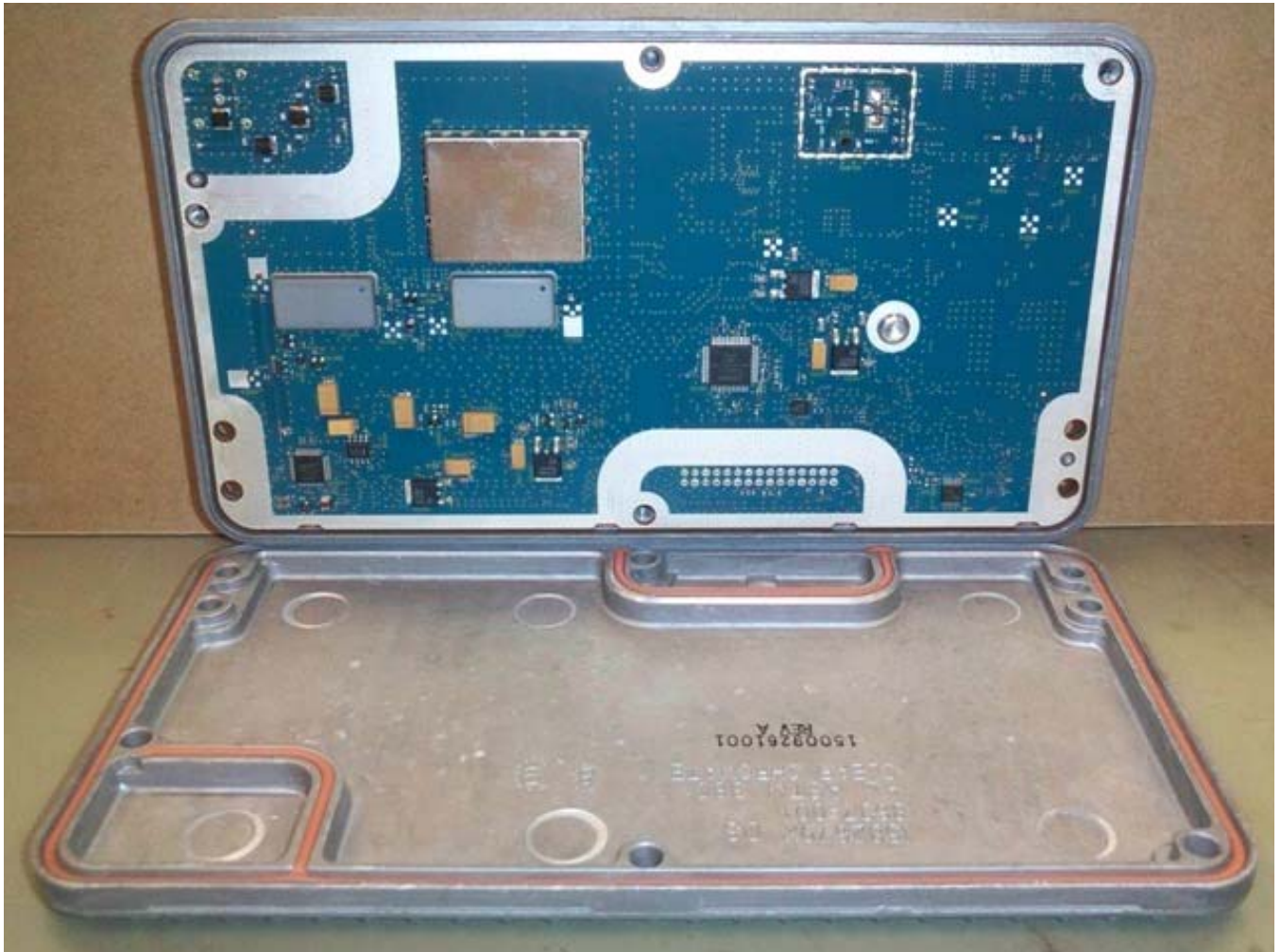
Internal Back View – Receiver Board, Bottom View
