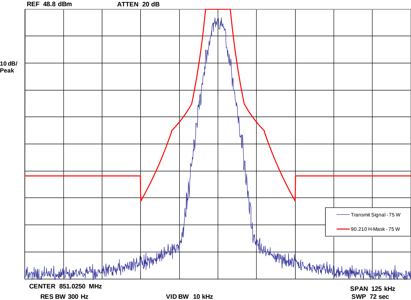
Occupied Bandwidth -- 4-Level Frequency Shift Keying Modulation - 75 Watts
