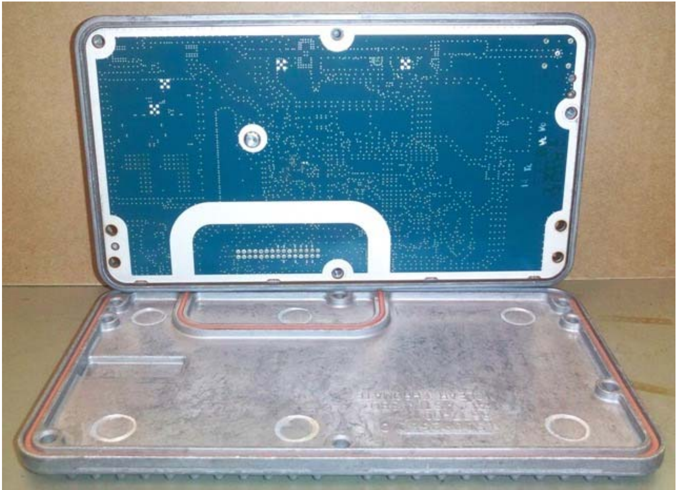
Internal Back View – Exciter Board, Bottom View
