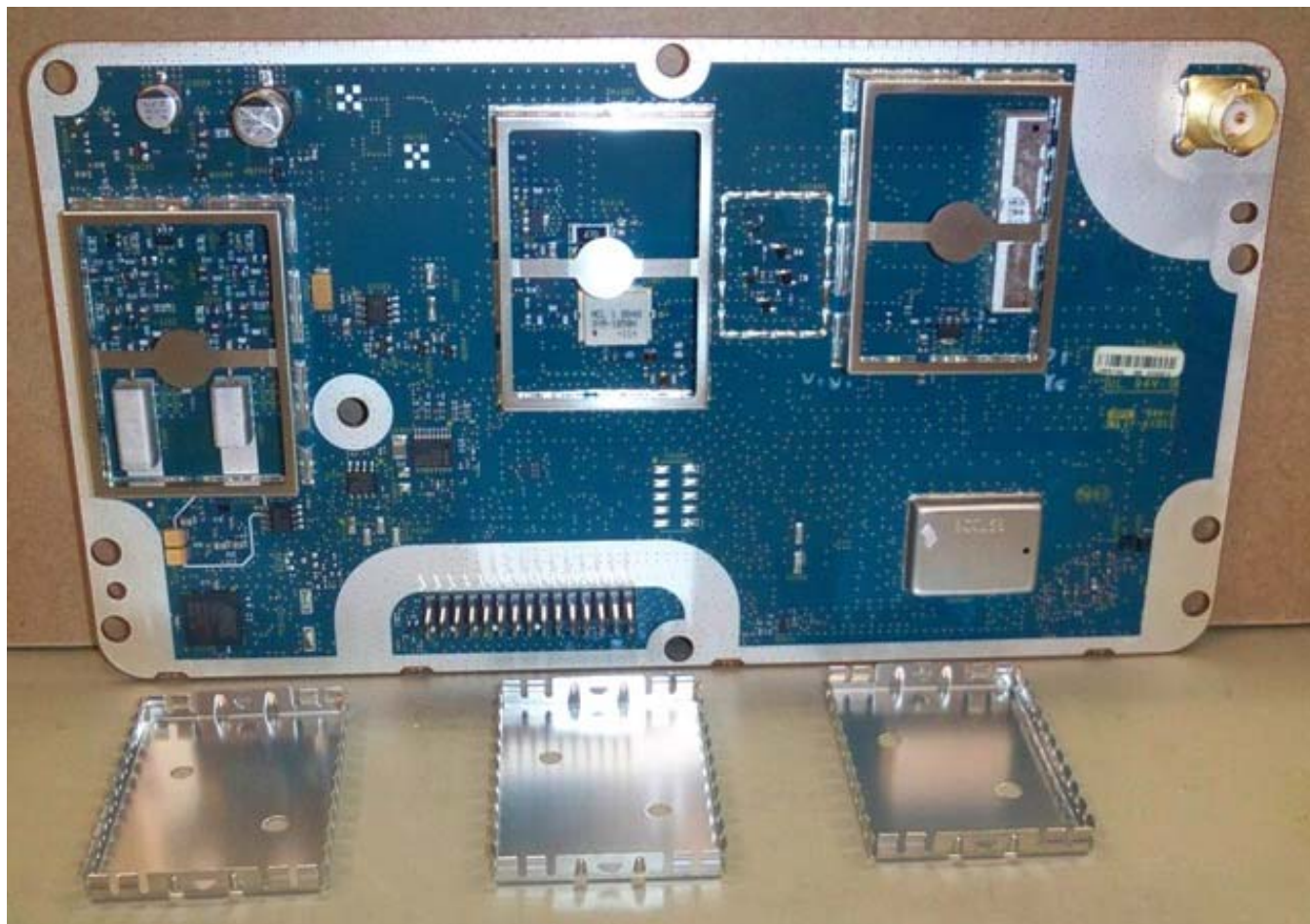
Internal Front View –Receiver Board, Top View
