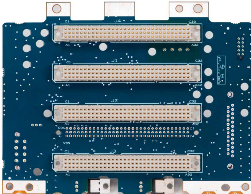
Internal Front View – Backplane
