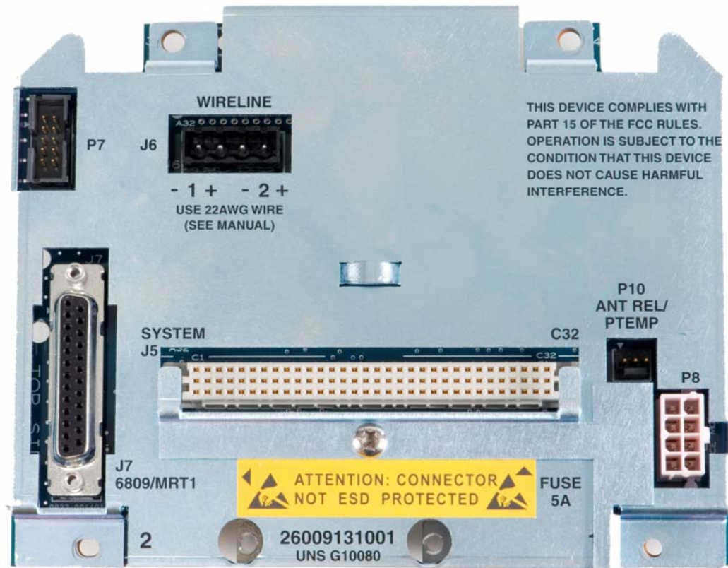
Internal Back View – Backplane
