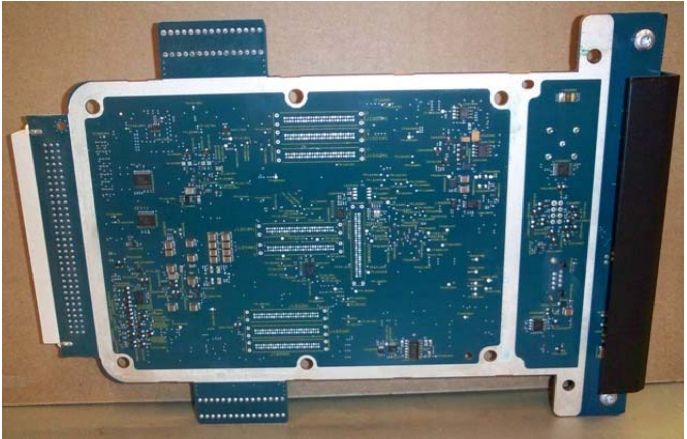
Internal Back View – Control Board, Bottom View
