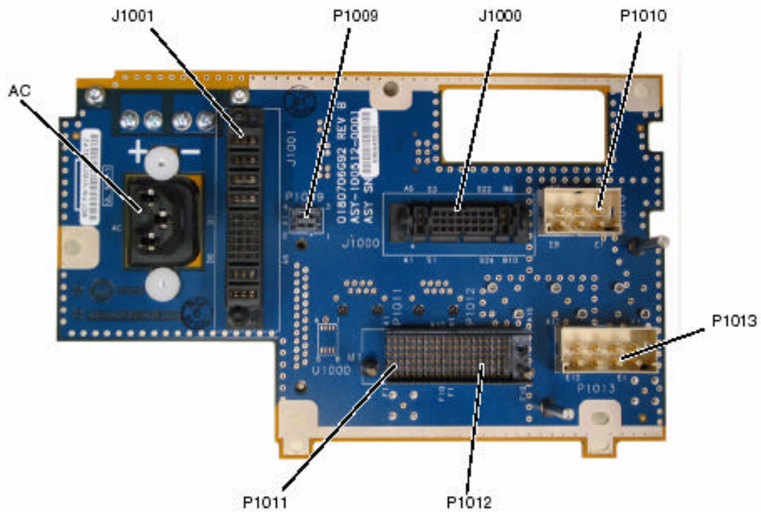
Internal Front View – Backplane
