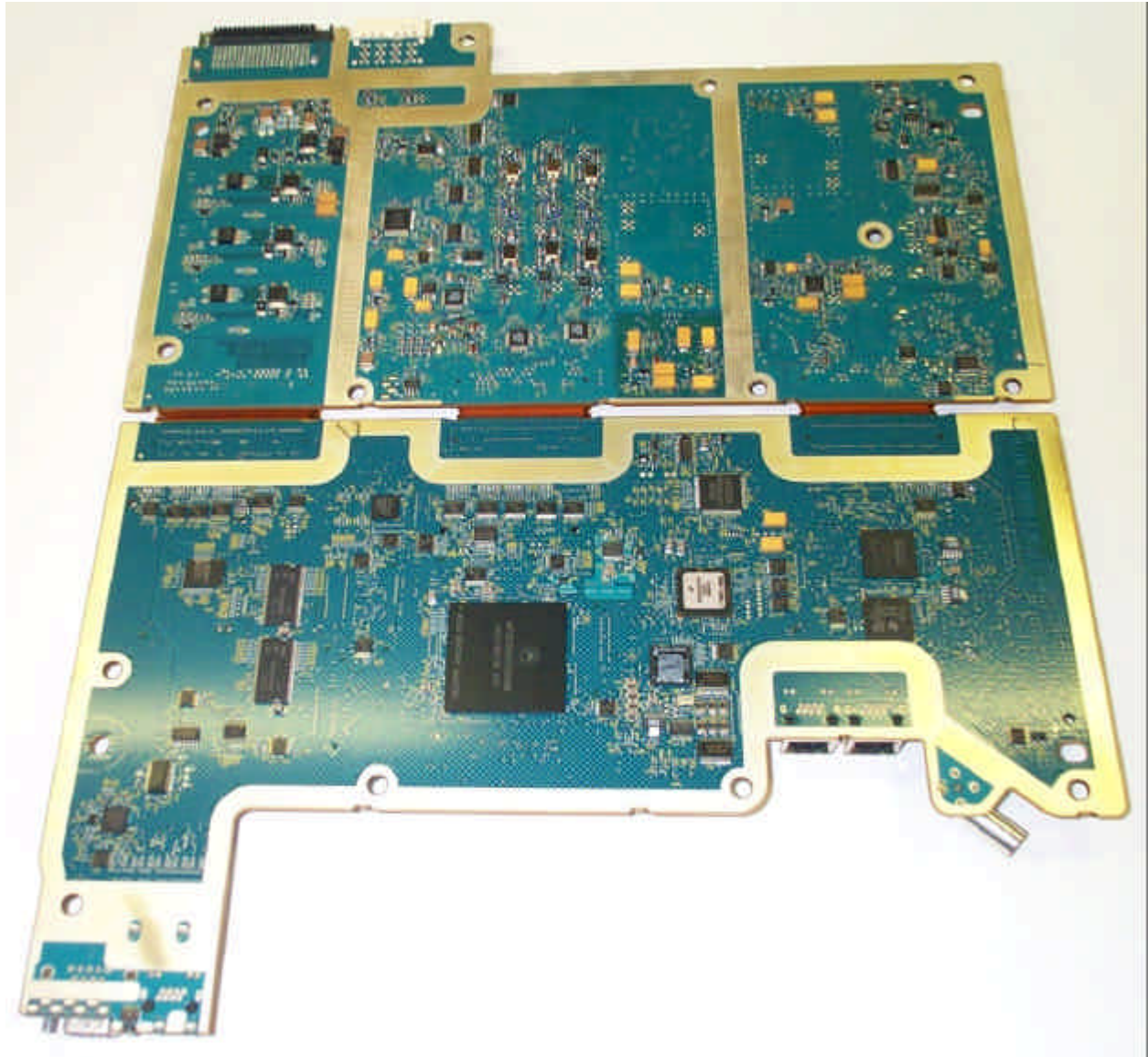
Internal Back View – Transceiver Module
