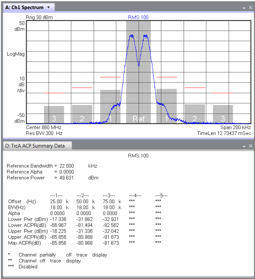
Figure 1 Two Carrier System Example ACP Test System Diagram, Limits, Example Output
