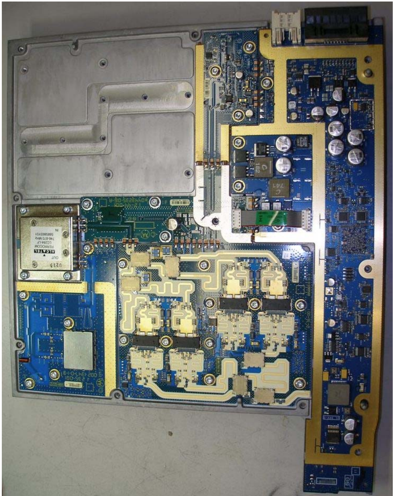
Internal Front View – Power Amplifier Module, Cover Removed
