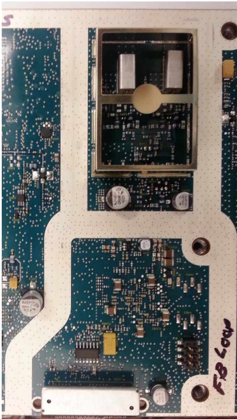
Internal Front View – Transceiver Module, Exciter Section
