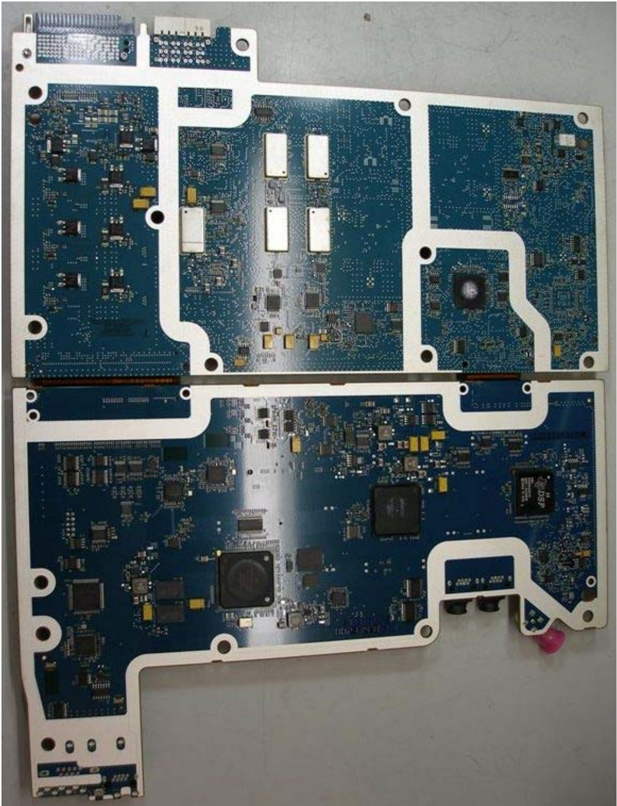
Internal Back View – Transceiver Module
