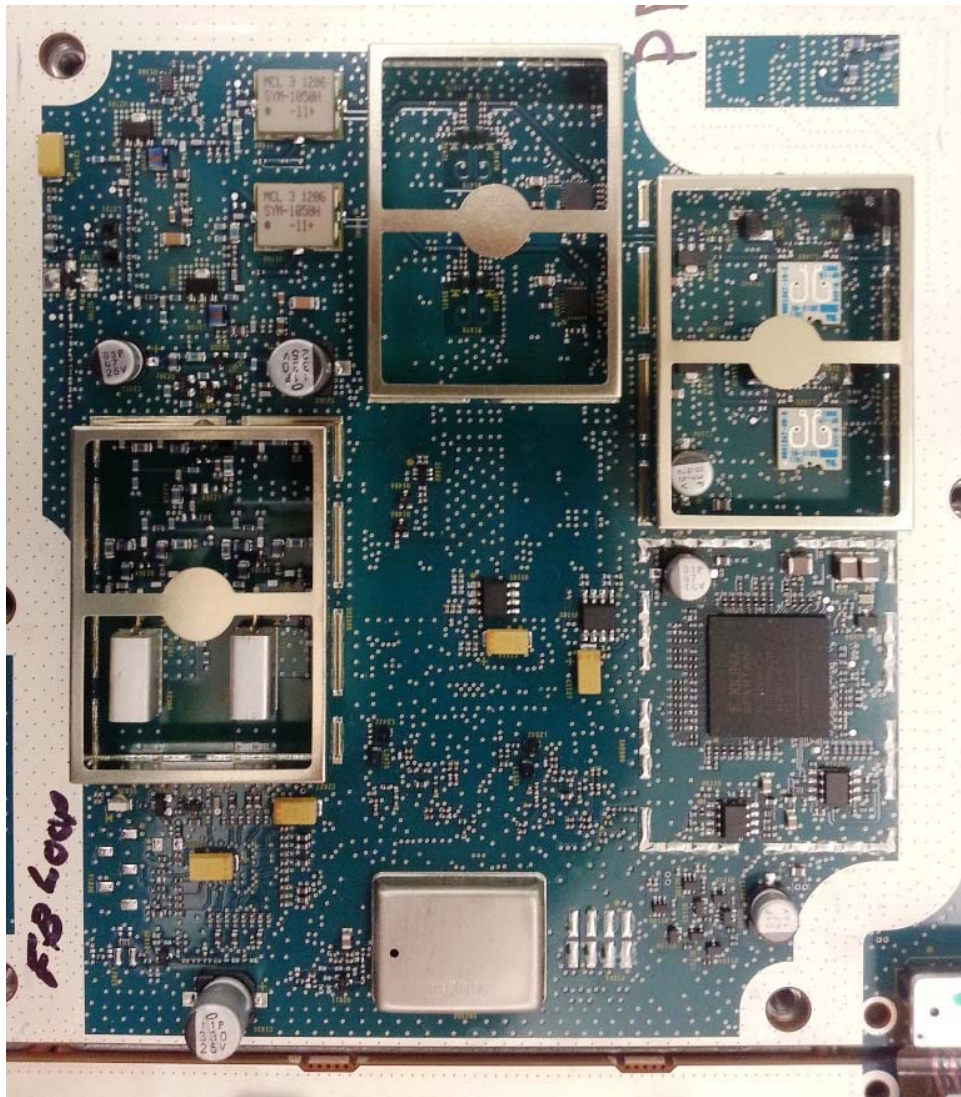
Internal Front View – Transceiver Module, Receiver Section
