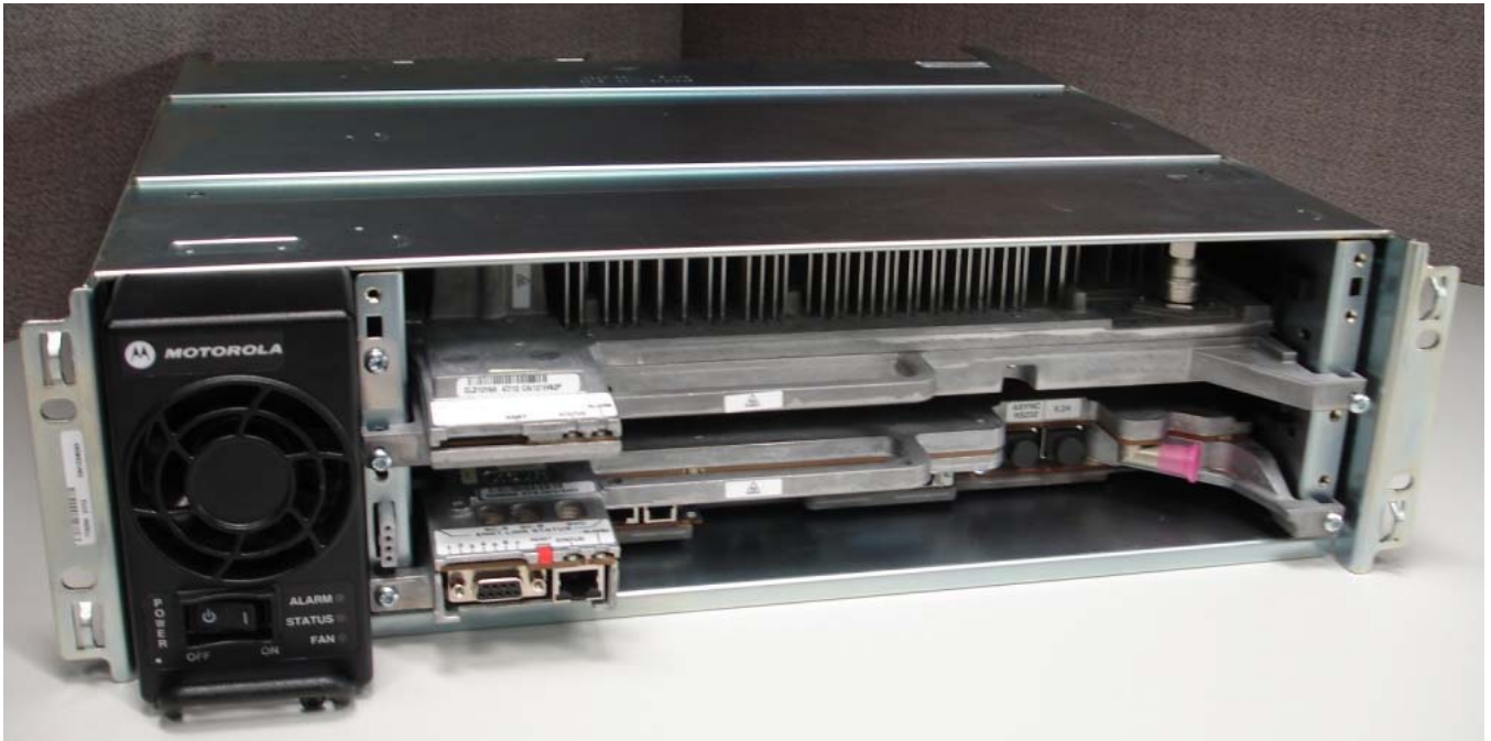
External Front View of Base Radio, Front Panel Removed
