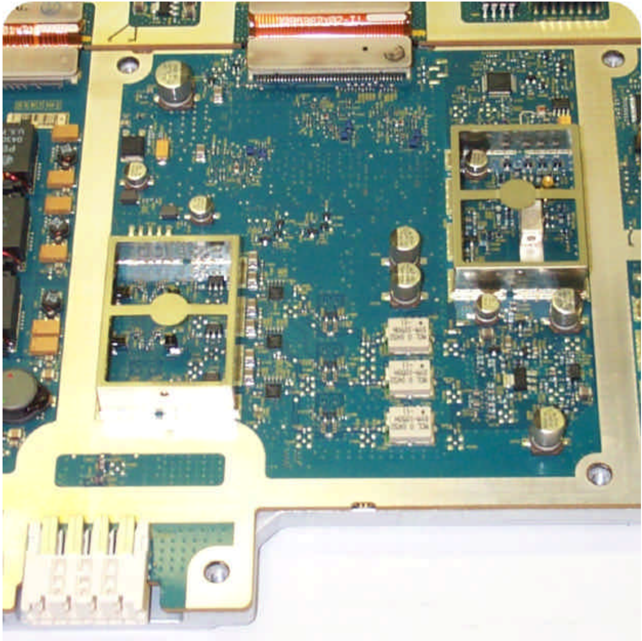
Internal Front View – Transceiver Module, Receiver Section
