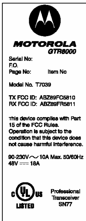
FCC Identification Label
