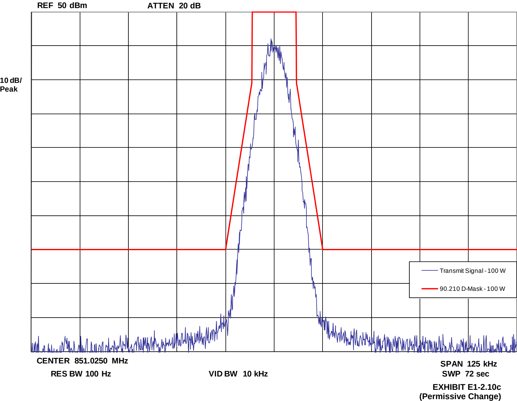
Occupied Bandwidth -- Compatible 4-Level Frequency Modulation - 100 Watts
