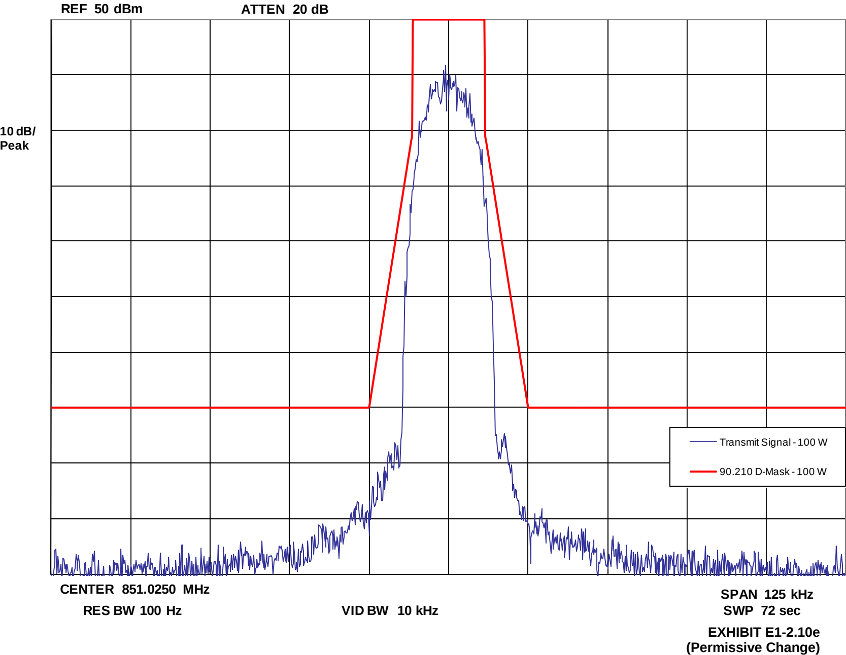
Occupied Bandwidth -- H-DQPSK P25 Two Slot TDMA Digital Modulation - 100 Watts (Average)
