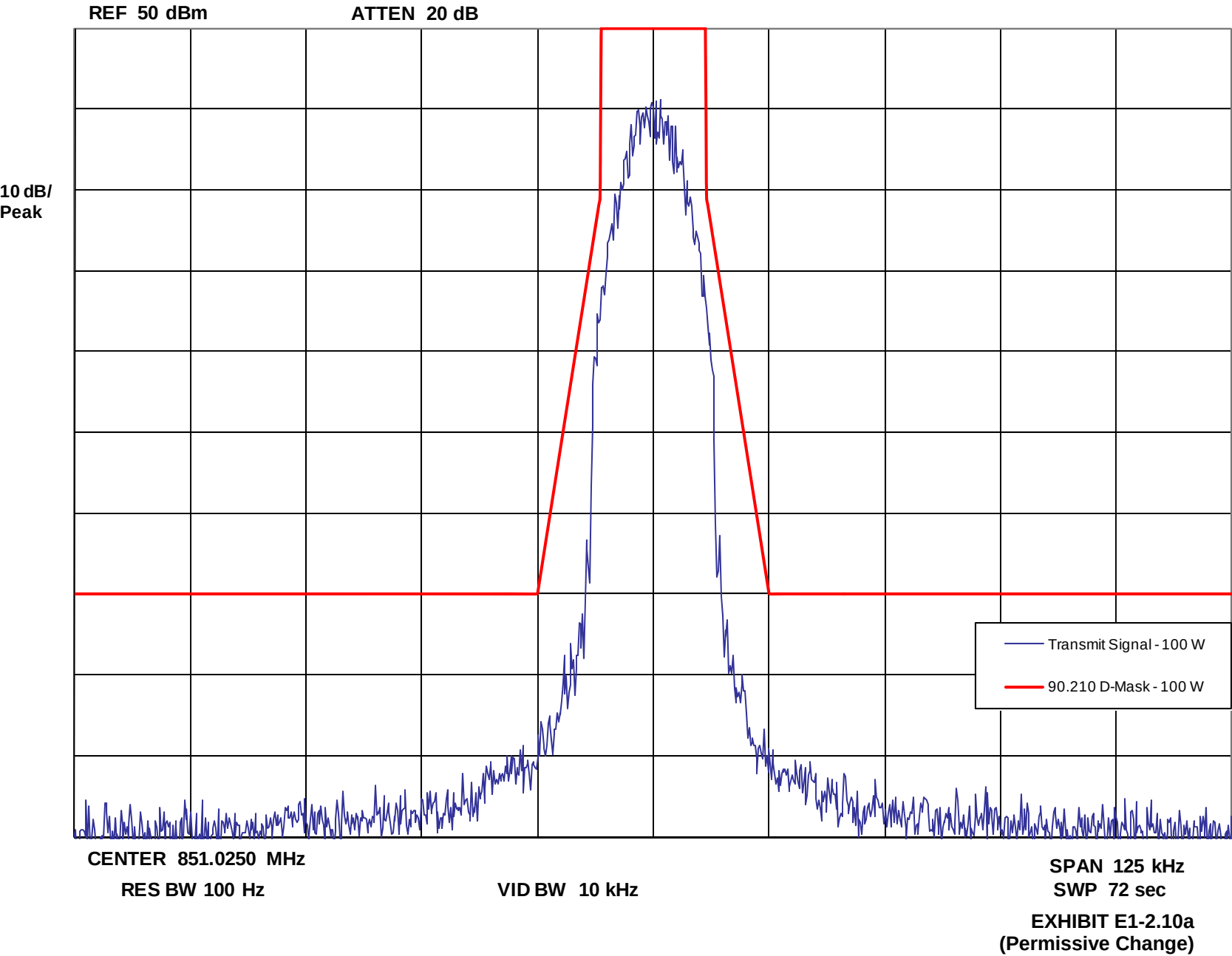
Occupied Bandwidth -- Linear Simulcast Modulation - 100 Watts (Average)
