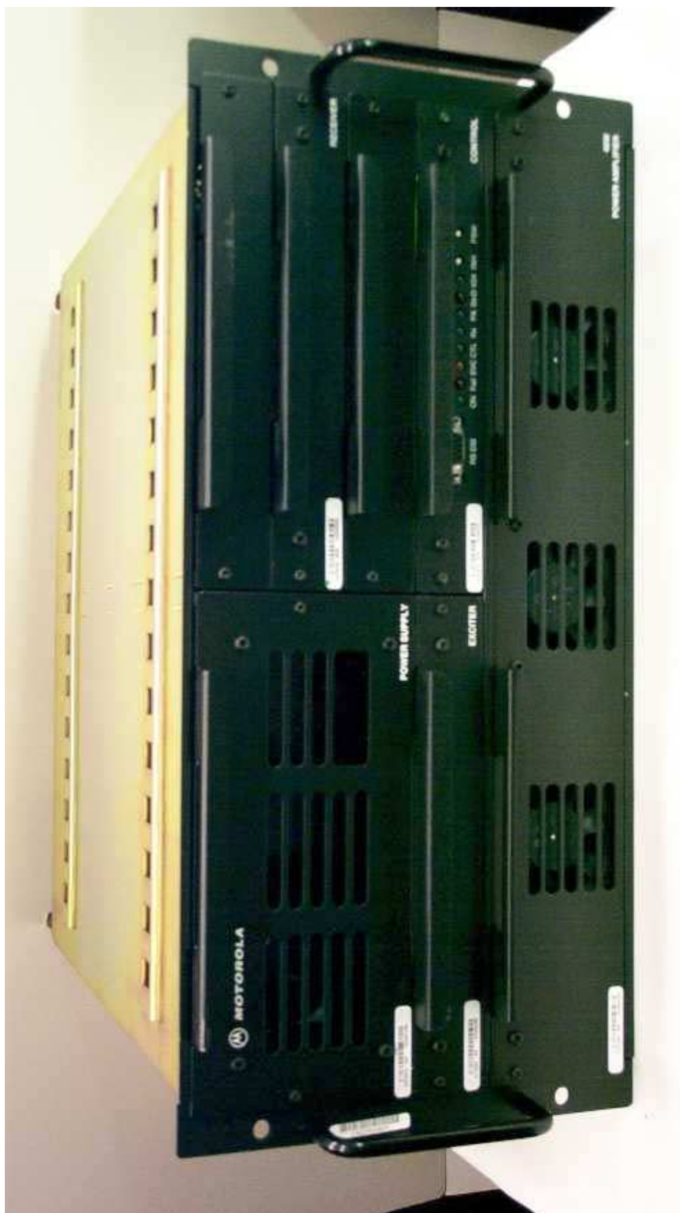
Linear Simulcast Station Base Radio -- Front View
