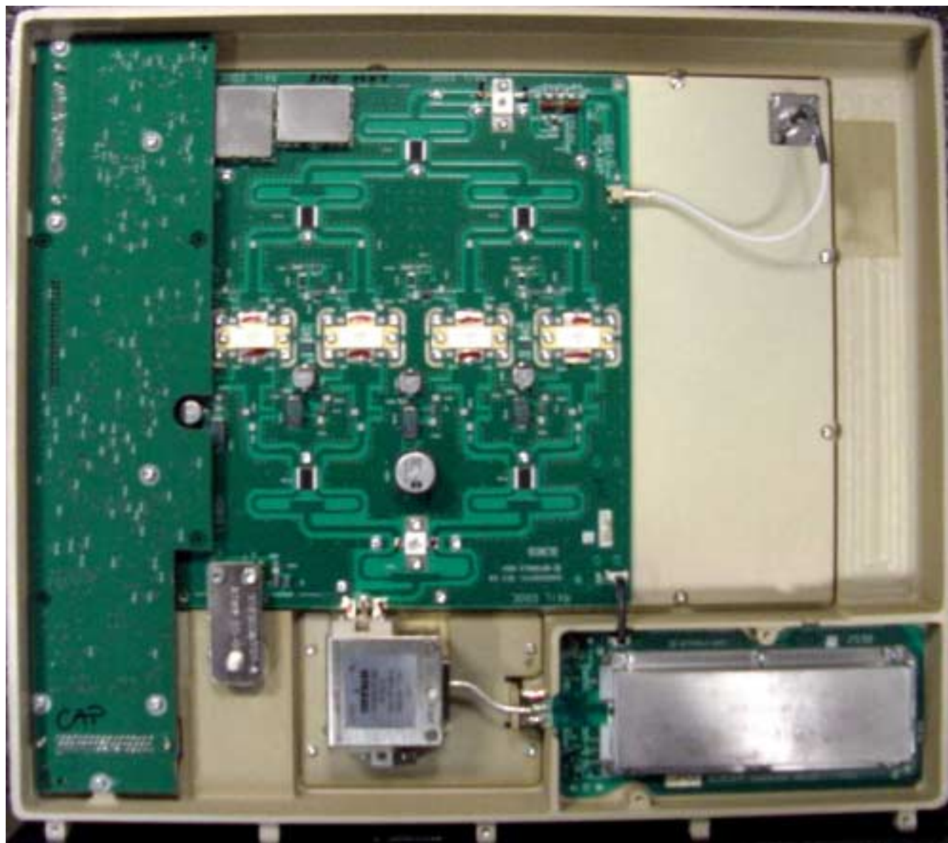
High Power Booster – Internal View
