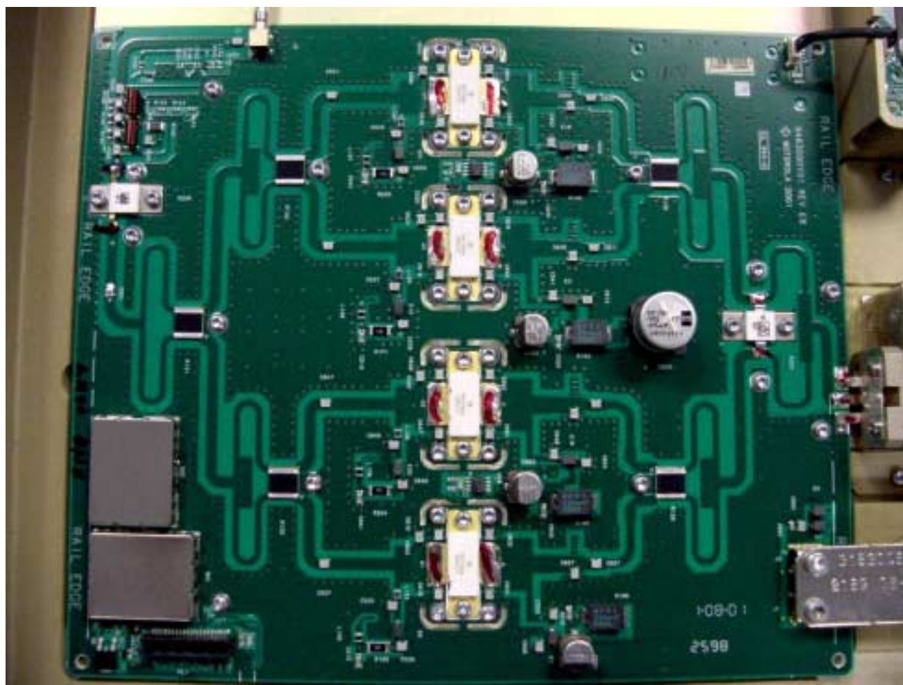
High Power Booster RF Board
