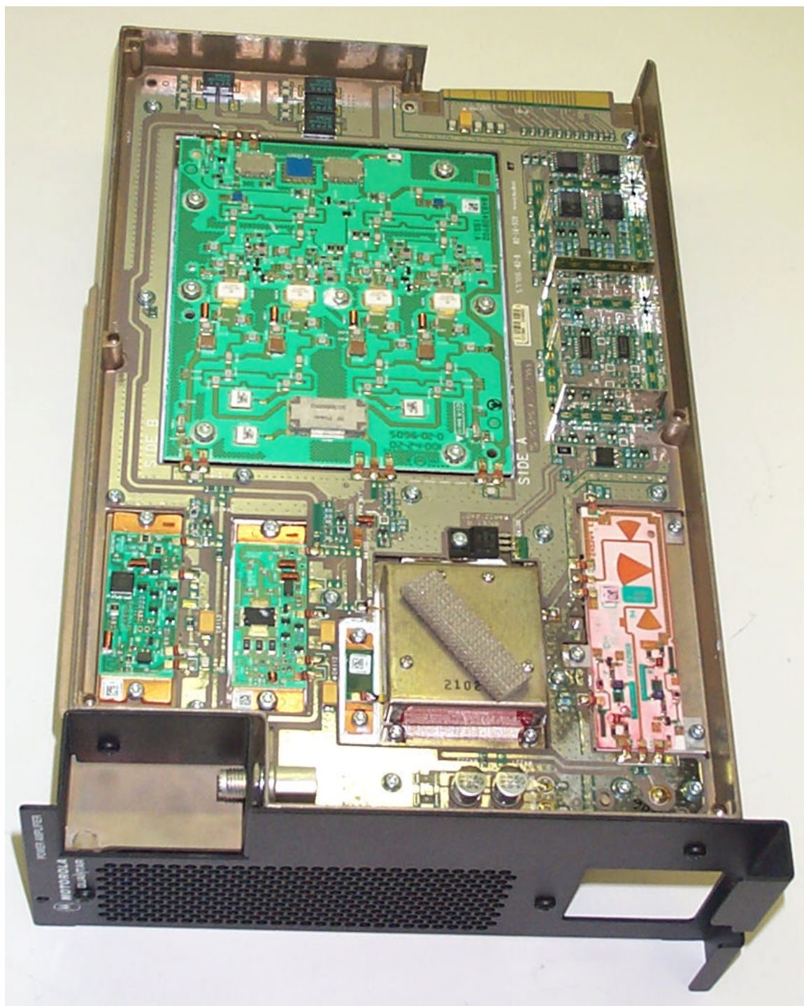
Power Amplifier Module, Top View, Shields Removed
