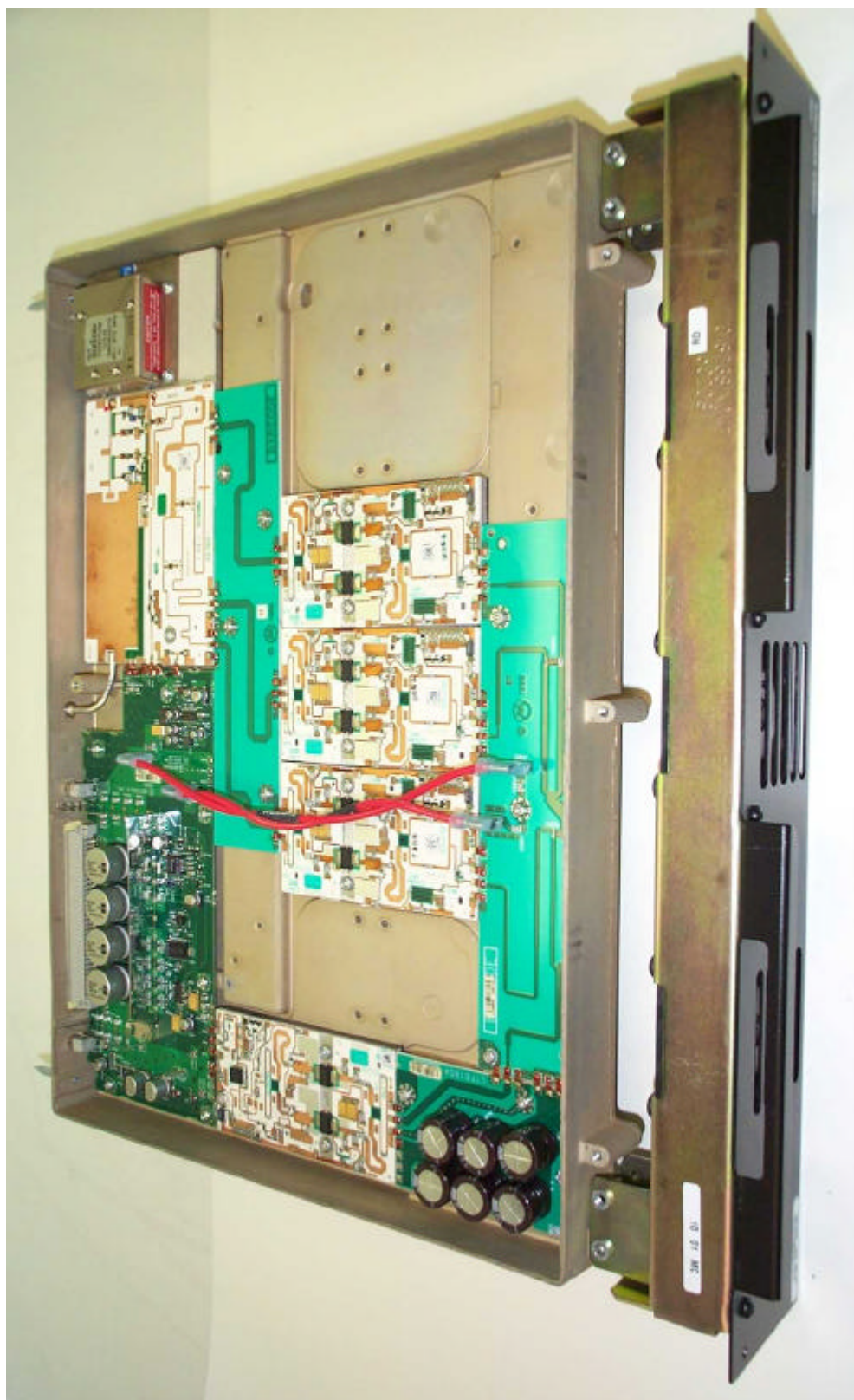
Power Amplifier Module, Top View, Shields Removed
