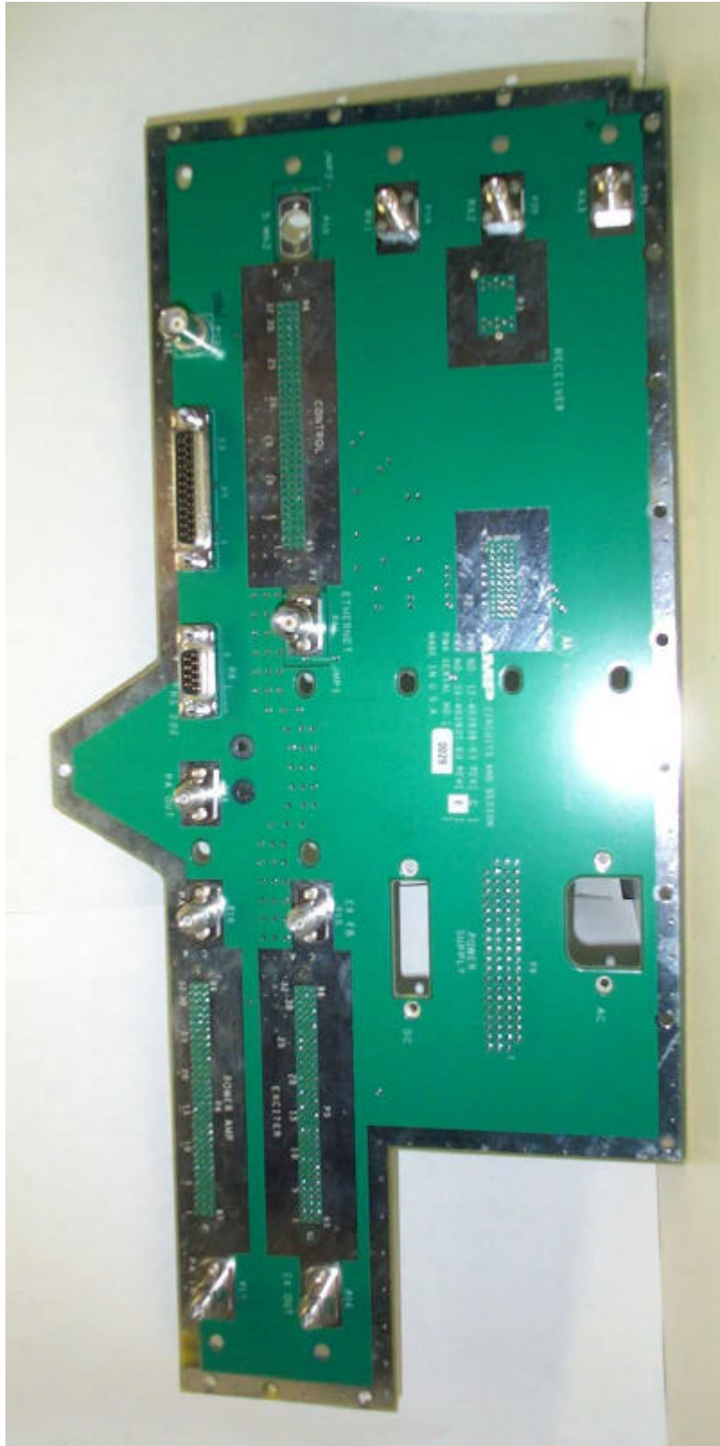
Backplane Board, Back Side
