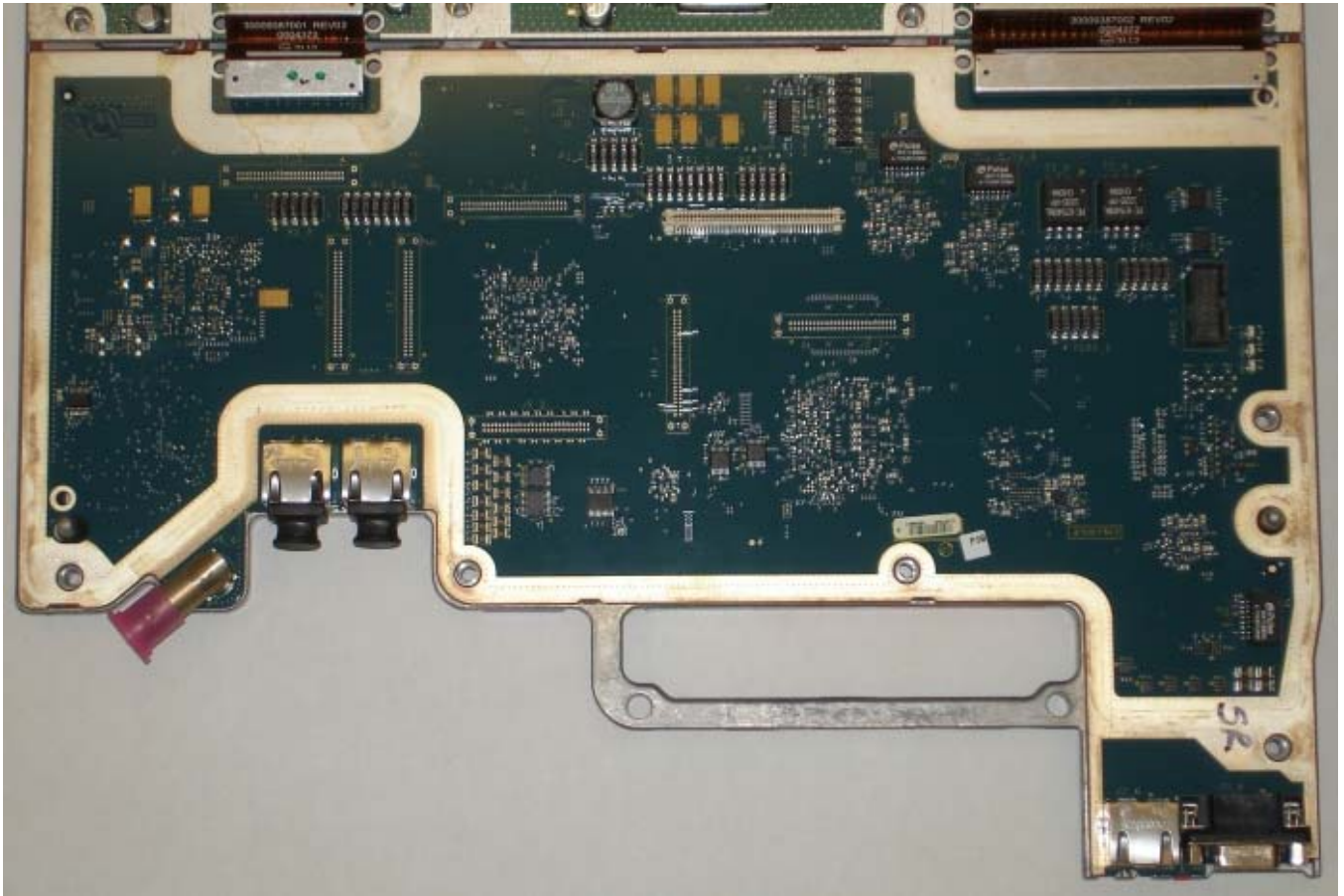
Internal Front View – Transceiver Module, Control Section
