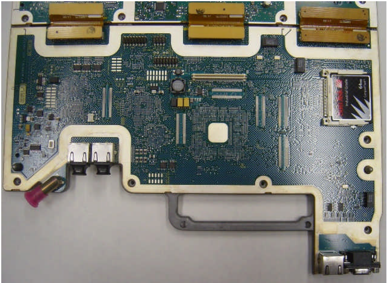
Internal Front View – Transceiver Module, Control Section
