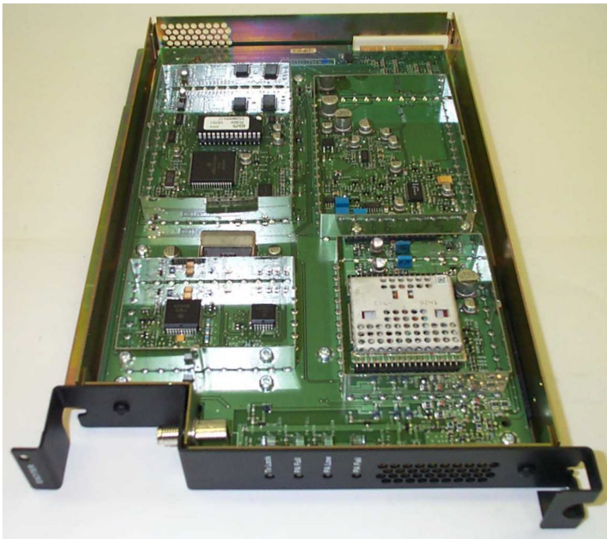
Exciter Module, Top Side – Range 2 Exciter Shown
