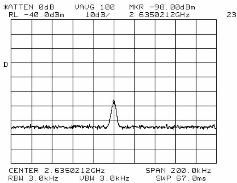
Plot 9: VCO Feedthrough, 3kHz RBW:
