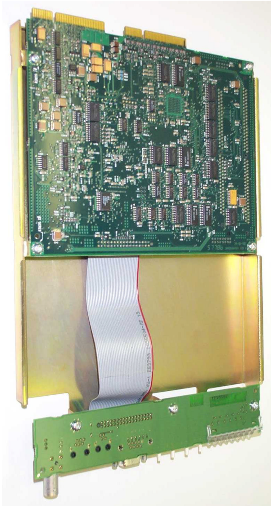
Control Module, Bottom Side
