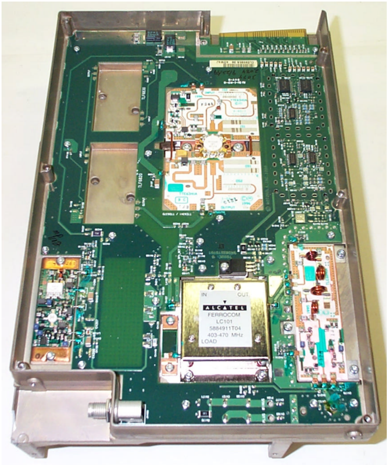
Power Amplifier Module, Top View, Shields Removed
