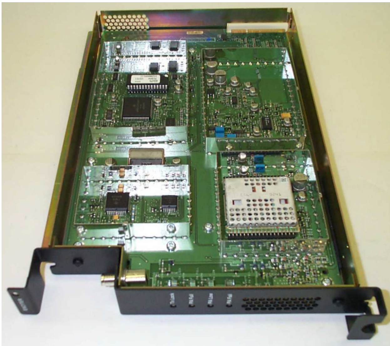
Exciter Module, Top Side
