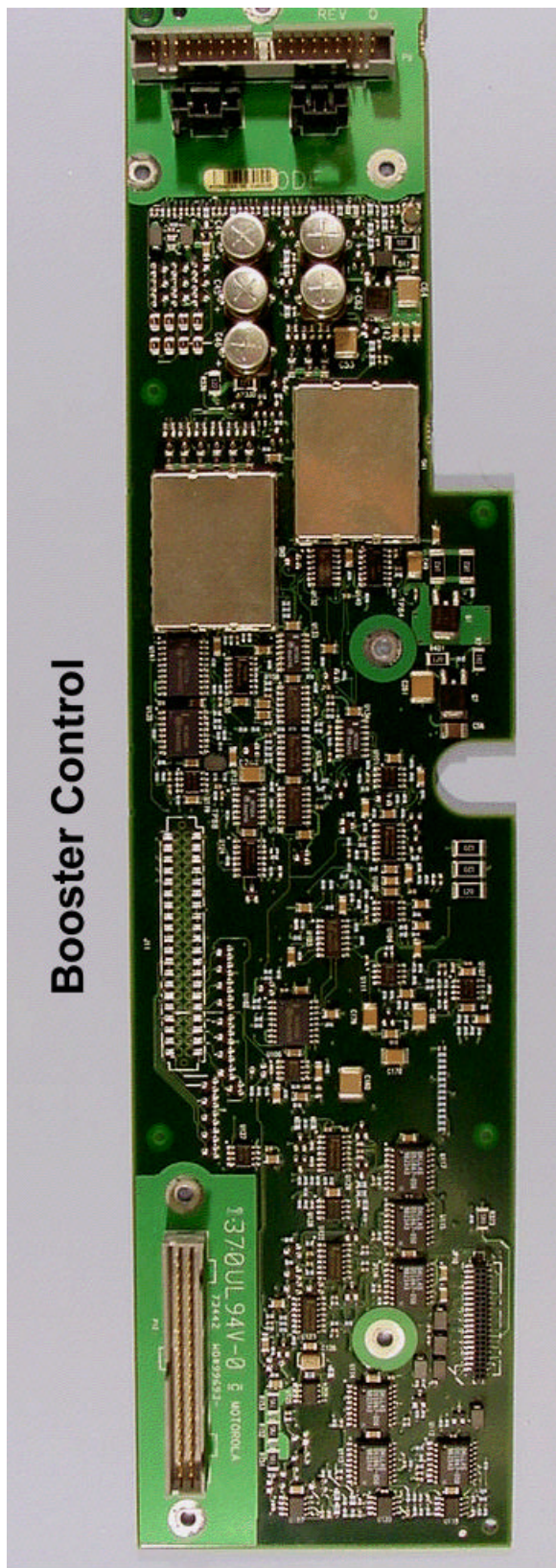
High Power Booster Control Board
