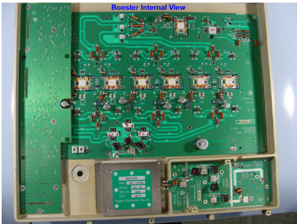
High Power Booster – Internal View
