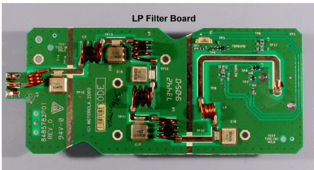
High Power Booster LPF Board
