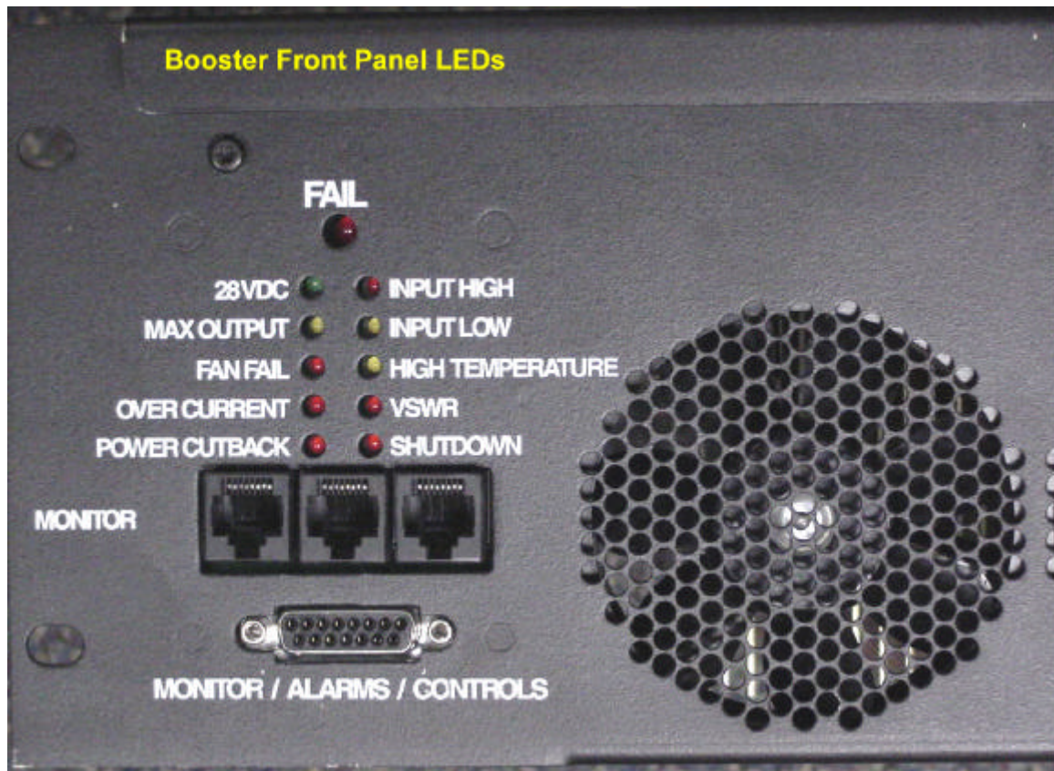
High Power Booster Front Panel LEDs
