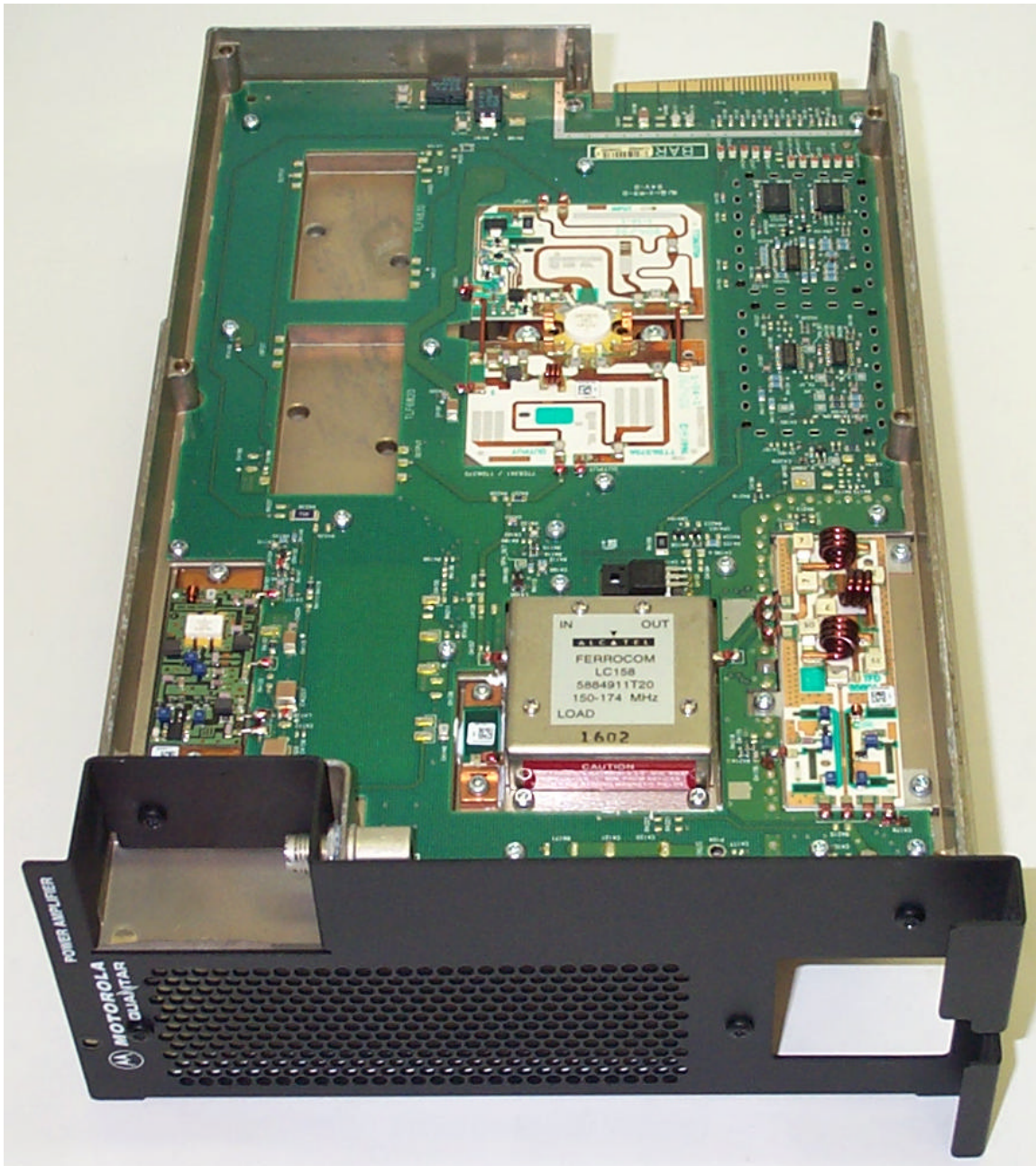
Power Amplifier Module, Top View, Shields Removed
