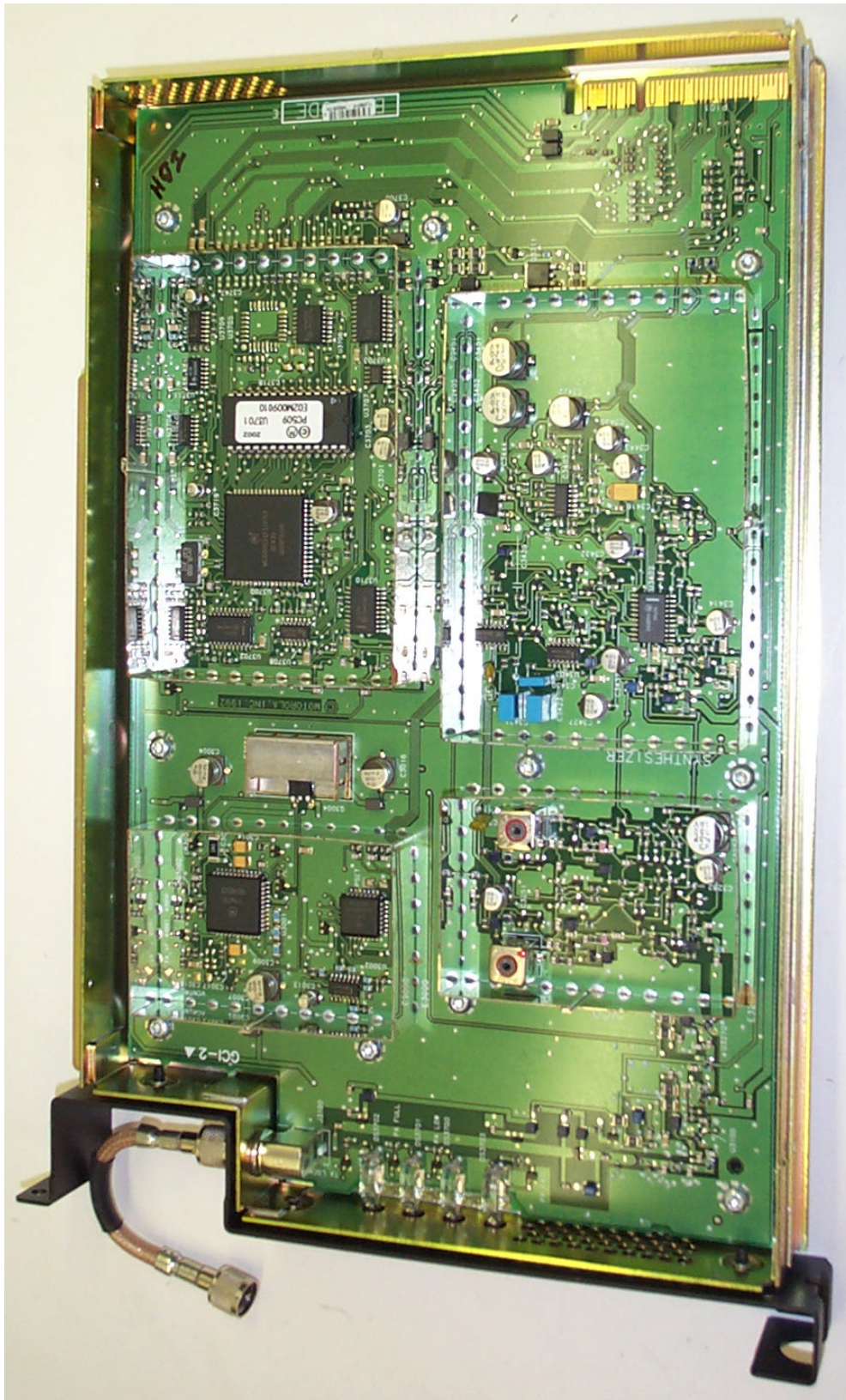
Exciter Module, Top Side
