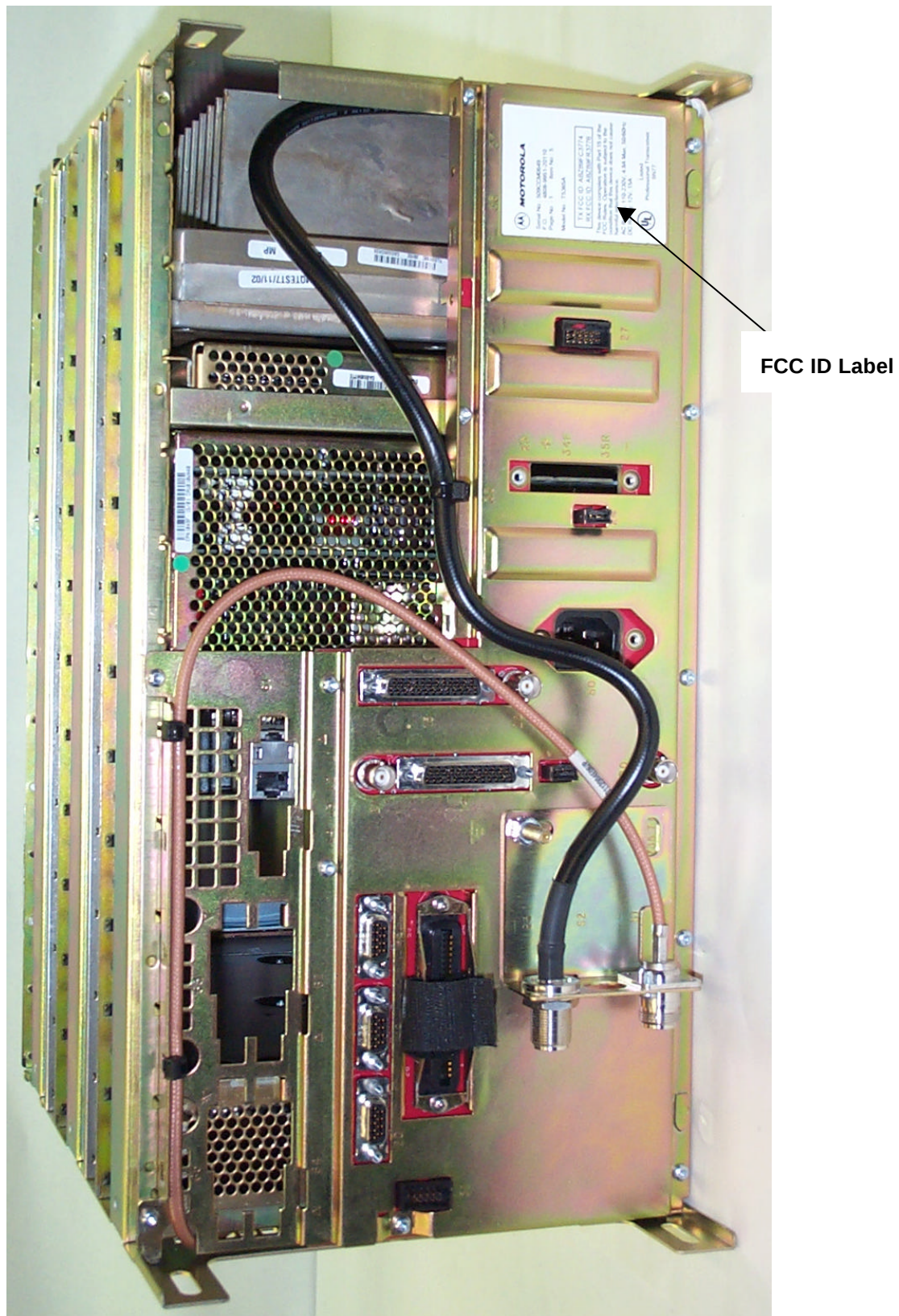
Rear of Base Radio Including Location of the FCC ID Label
