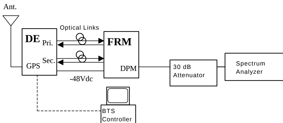
Figure 4: Test Setup for Antenna Port Spurious Emission Measurement
