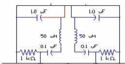
Figure 3-4. LISN Schematic Diagram
