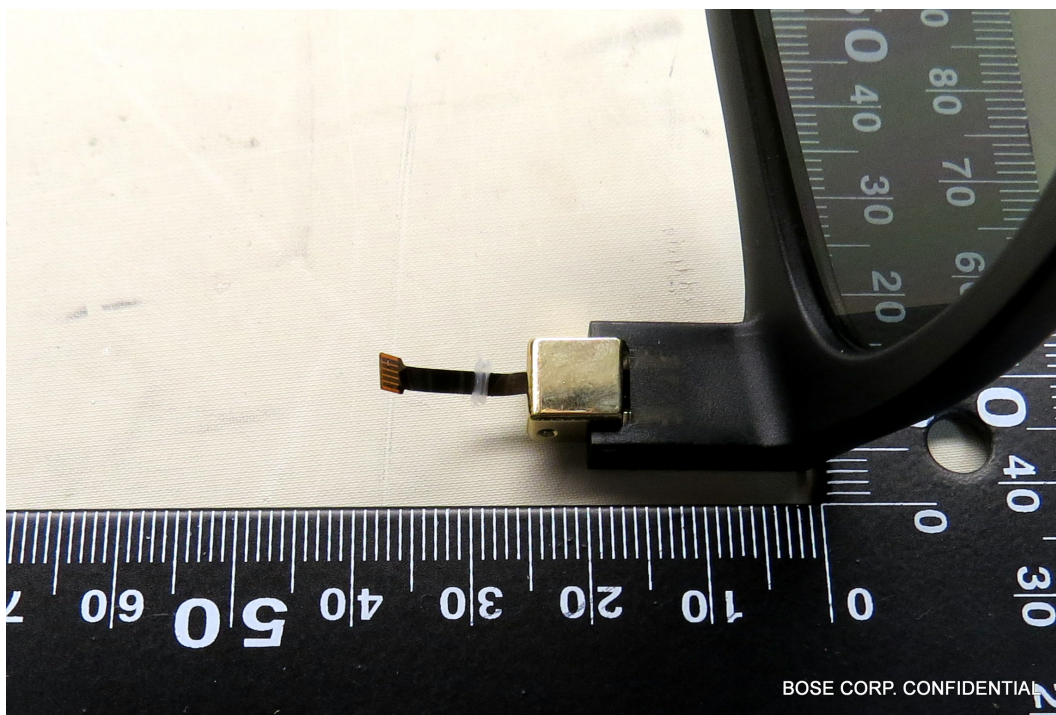
Right temple FFC connection (FFC is molded into the lens frame)
