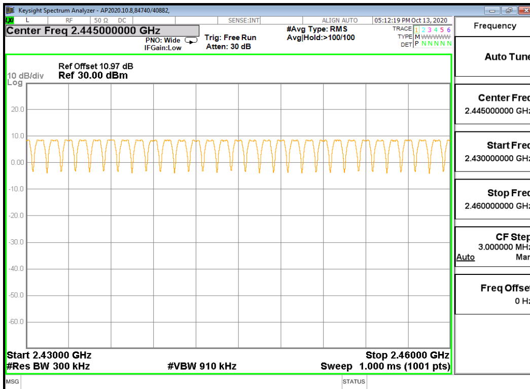
30MHz SPAN, SEGMENT 2 OF 3
