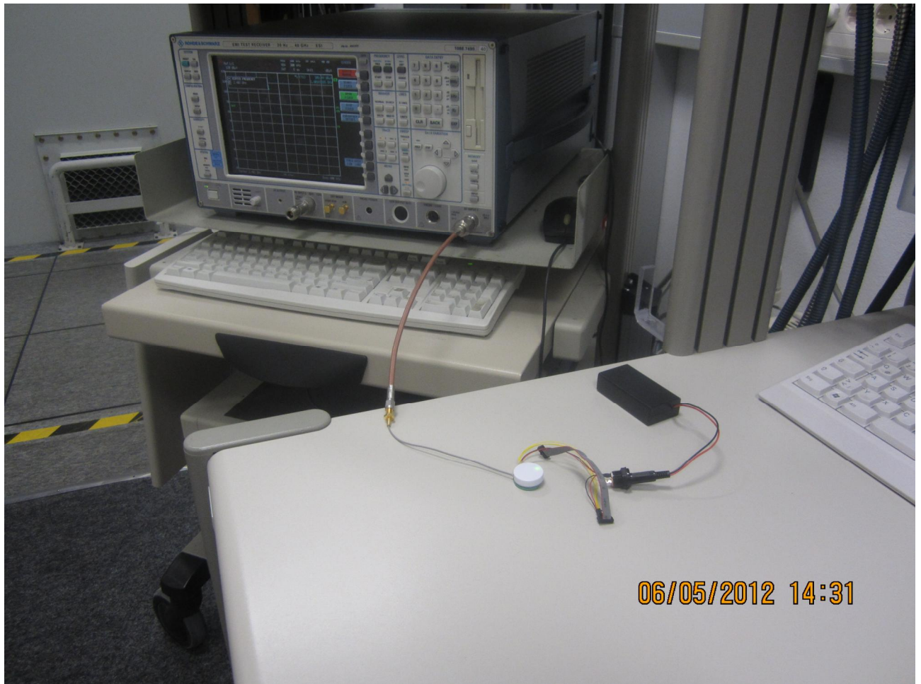
120795_5.JPG: Test set-up conducted measurement
