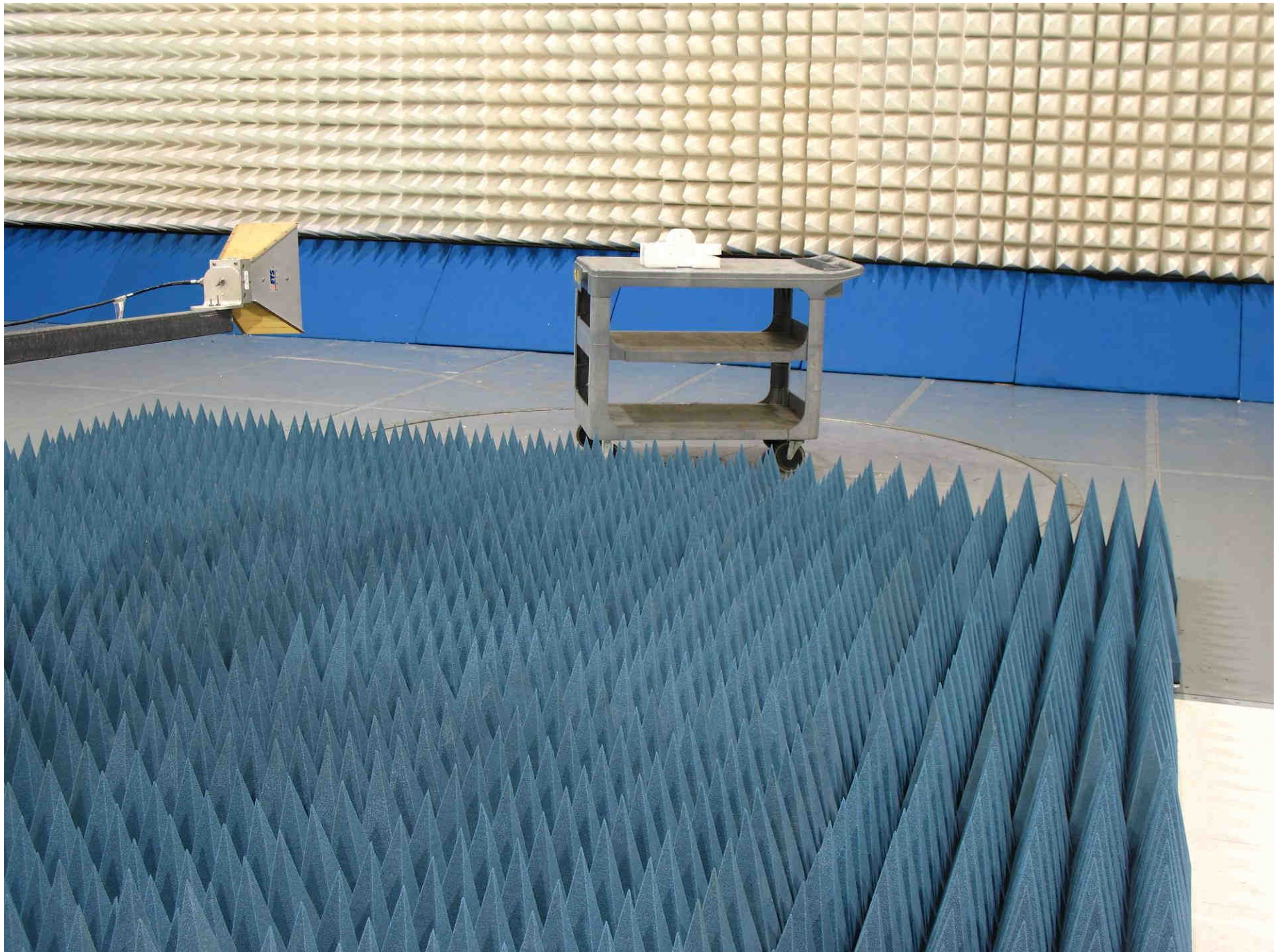
Radiated Testing (Front)
