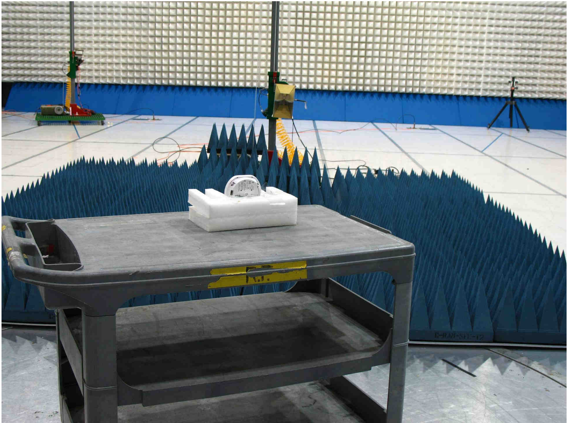
Radiated Testing (Back)
