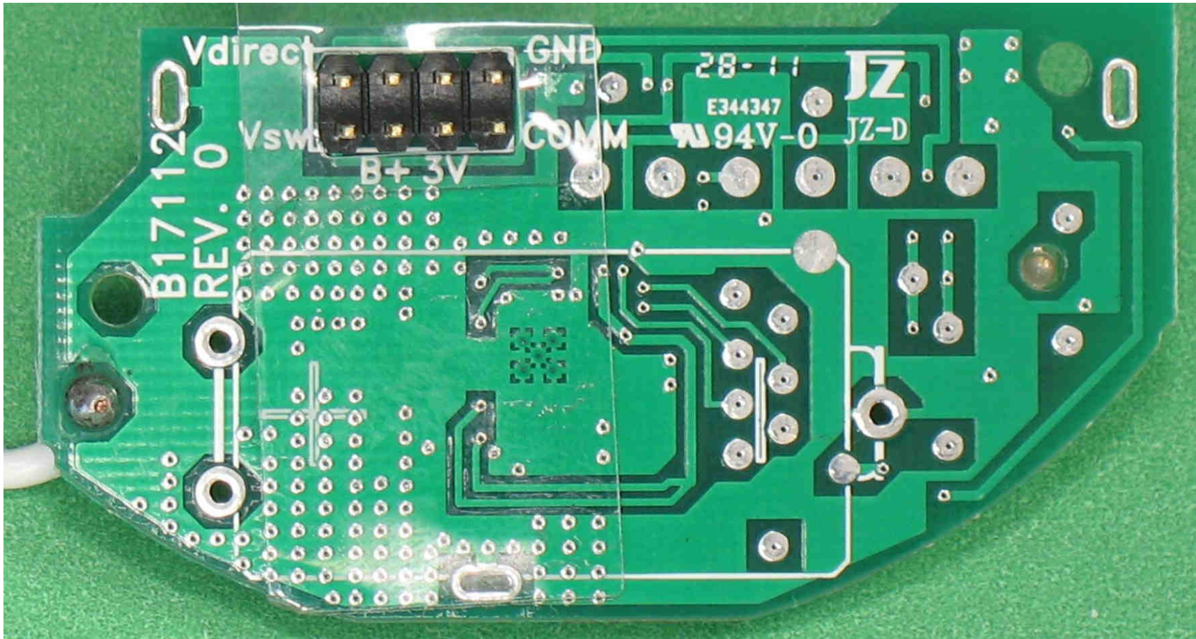
Back Side
