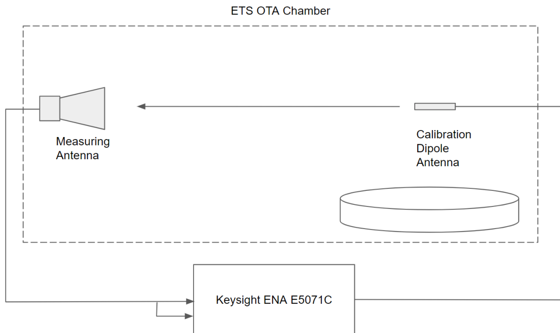
Figure: Chamber Block Diagram of Path Loss
