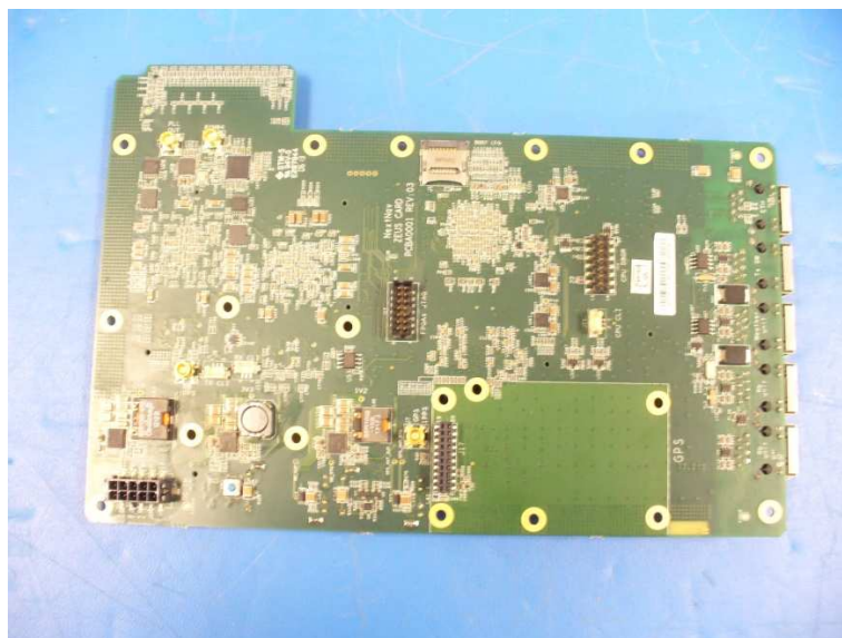
BOTTOM VIEW
