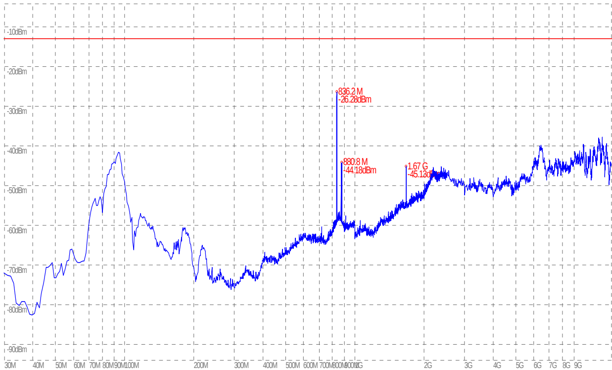
(Plot C.3: EGPRS 850MHz Channel = 190, Test Antenna Horizontal)
