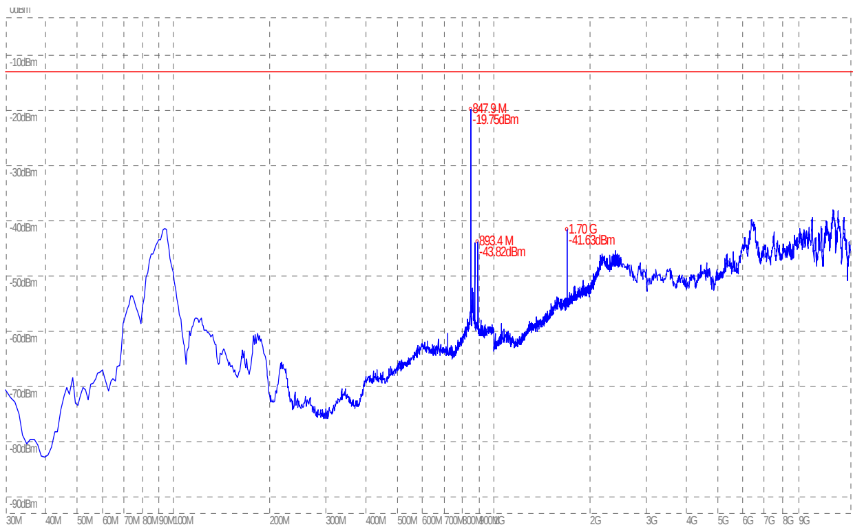
(Plot C.5: EGPRS 850MHz Channel = 251, Test Antenna Horizontal)
