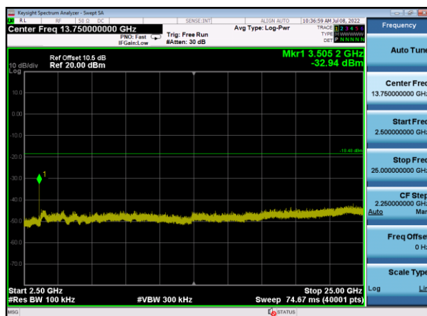
,Plot ,4Transmitter Spurious Emission : 2480,2500MHz~25000MHz
