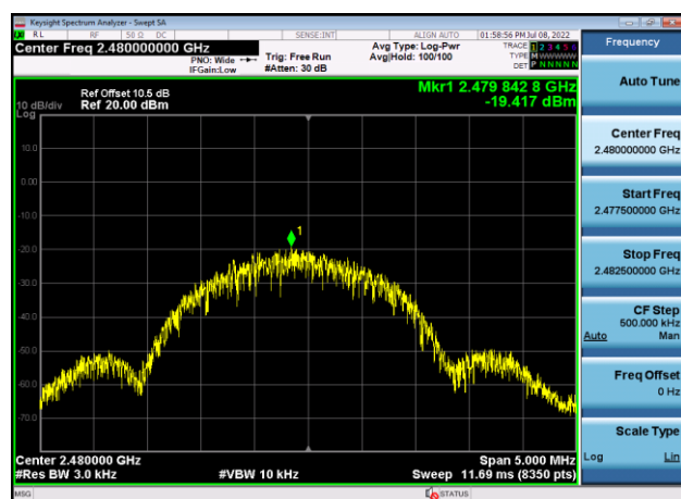
PSD: 2480MHz – 2MHz bandwidth
