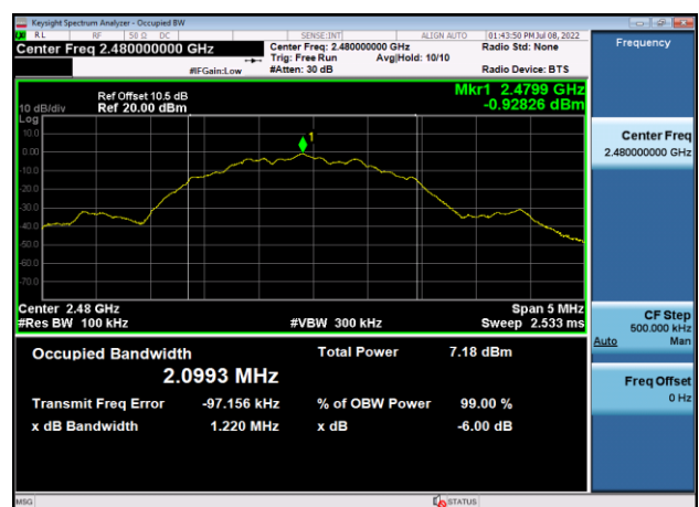
6dB Bandwidth: 2480MHz – 2MHz bandwidth
