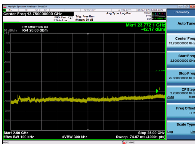
,Plot ,4Transmitter Spurious Emission : 2440,2500MHz~25000MHz
