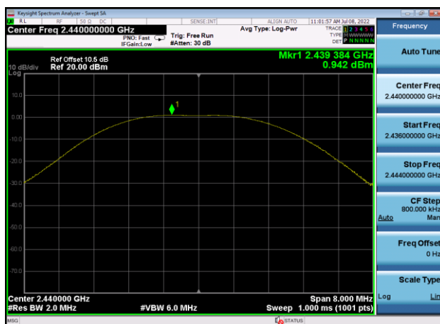
Output Power: 2440MHz – 2MHz bandwidth
