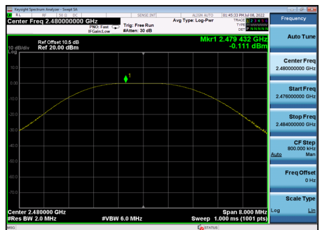
Output Power: 2480MHz – 2MHz bandwidth
