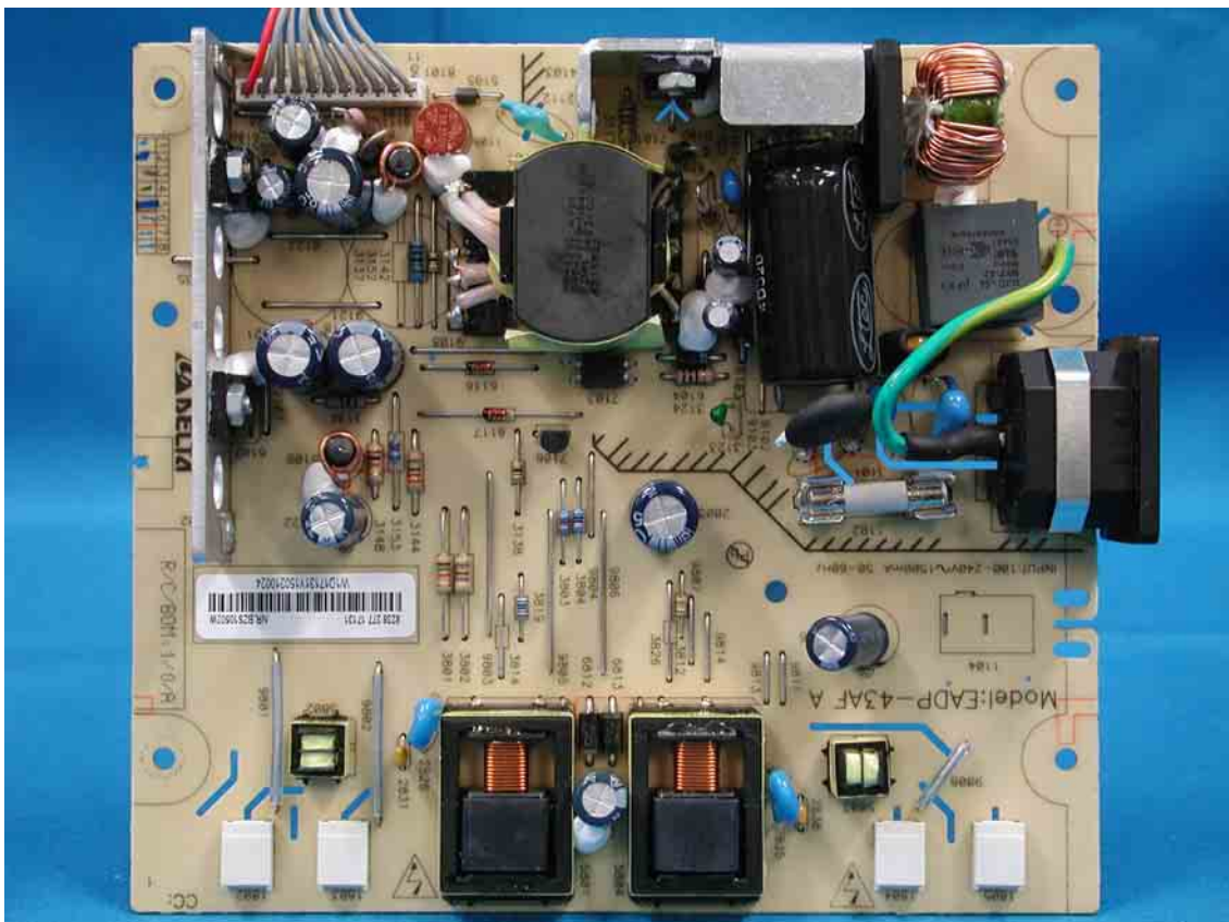
PCB Layout (Delta Power)
