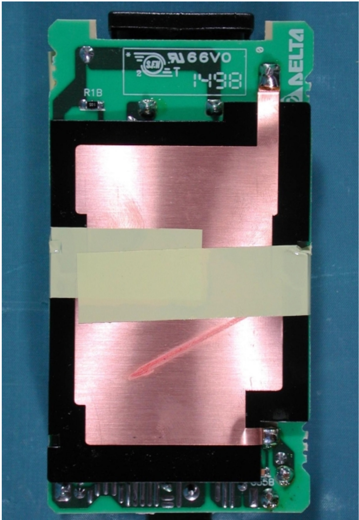
Assembly W/O Cabinet (Rear)
