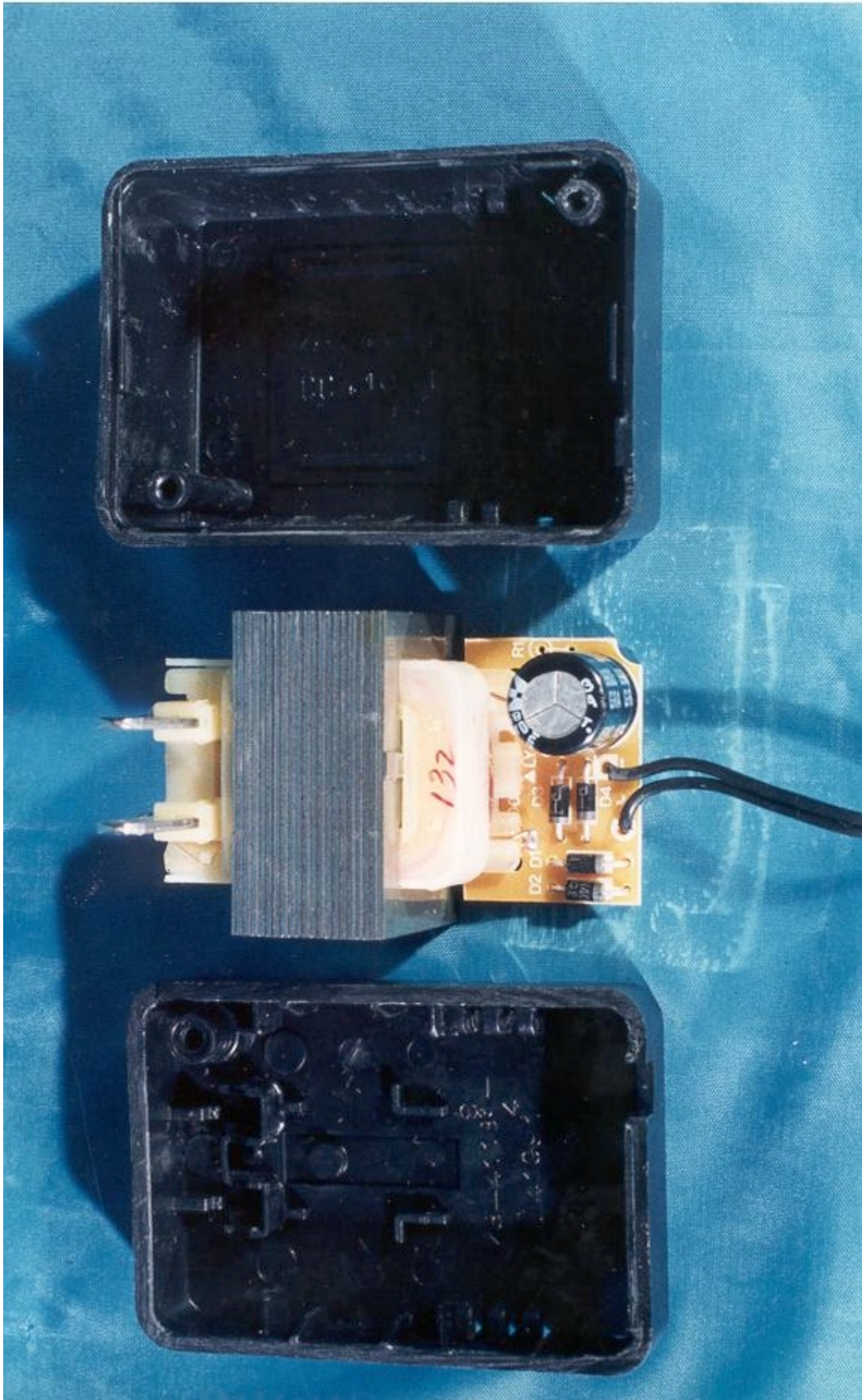
AC Adapter
