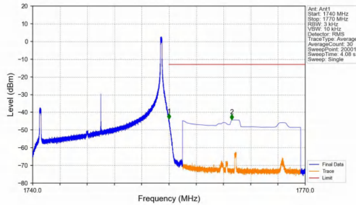
Band4_15MHz_16QAM_HCH_1747.5MHz_RB_1_74_NTNV
