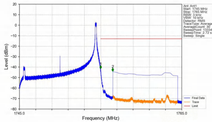
Band4_10MHz_16QAM_HCH_1750MHz_RB_1_49_NTNV
