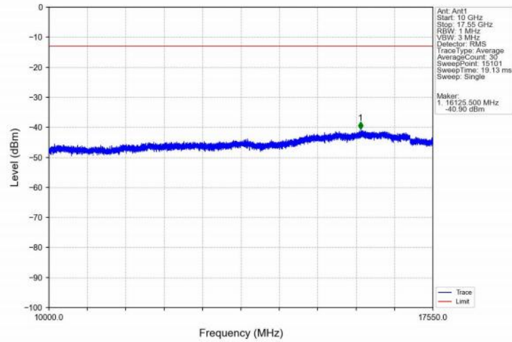
Band4_3MHz_16QAM_HCH_1753.5MHz_RB_1_0_NTNV
