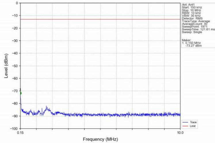
Band4_10MHz_16QAM_MCH_1732.5MHz_RB_1_0_NTNV
