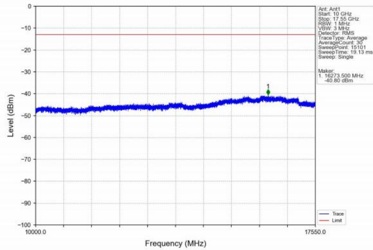
Band4_15MHz_16QAM_MCH_1732.5MHz_RB_1_0_NTNV
