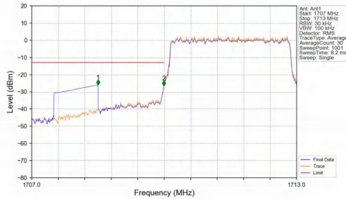
Band4_3MHz_16QAM_LCH_1711.5MHz_RB_15_0_NTNV
