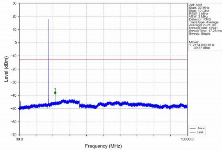
Band4_3MHz_16QAM_HCH_1753.5MHz_RB_1_0_NTNV
