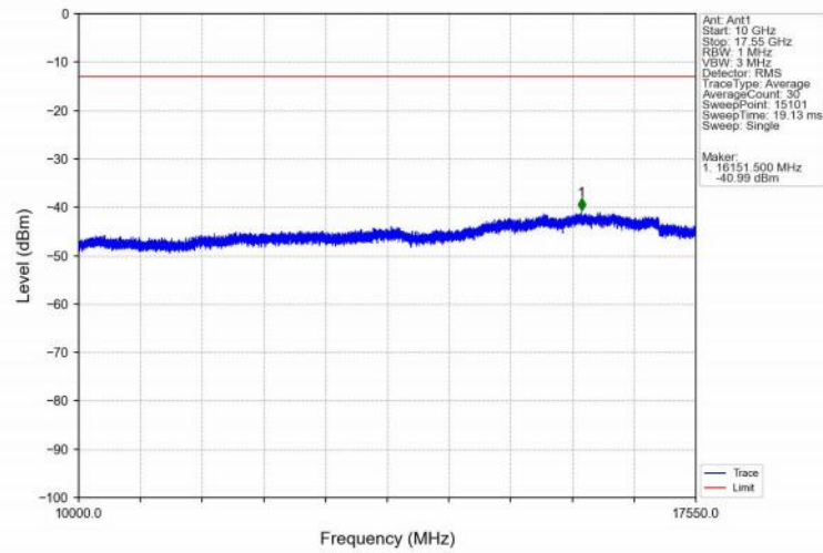
Band4_5MHz_QPSK_HCH_1752.5MHz_RB_1_24_NTNV
