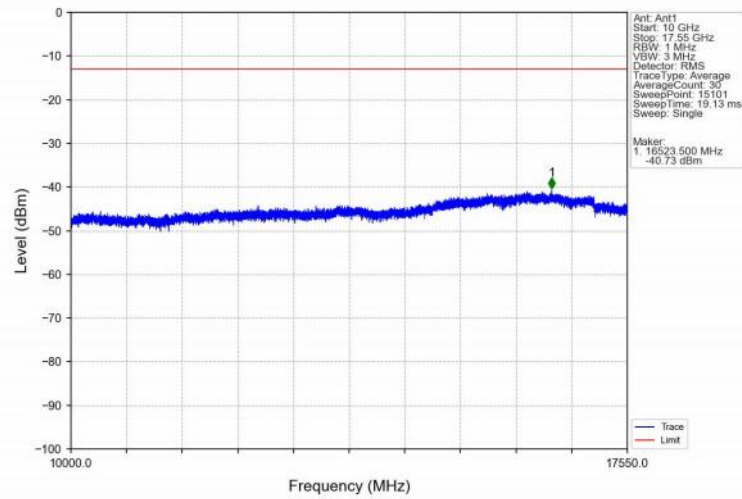
Band4_10MHz_16QAM_HCH_1750MHz_RB_1_49_NTNV
