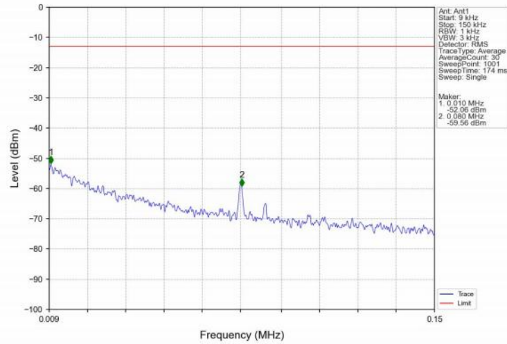
Band4_10MHz_16QAM_LCH_1715MHz_RB_1_0_NTNV
