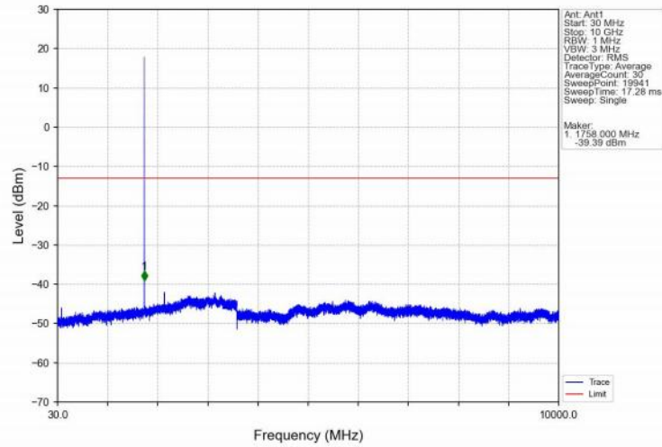
Band4_1.4MHz_16QAM_HCH_1754.3MHz_RB_1_0_NTNV
