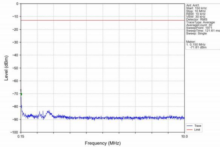
Band4_5MHz_QPSK_MCH_1732.5MHz_RB_1_0_NTNV
