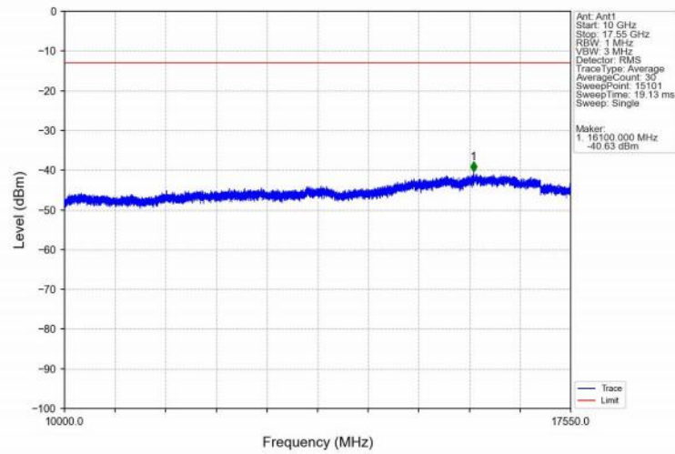
Band4_15MHz_16QAM_HCH_1747.5MHz_RB_1_74_NTNV
