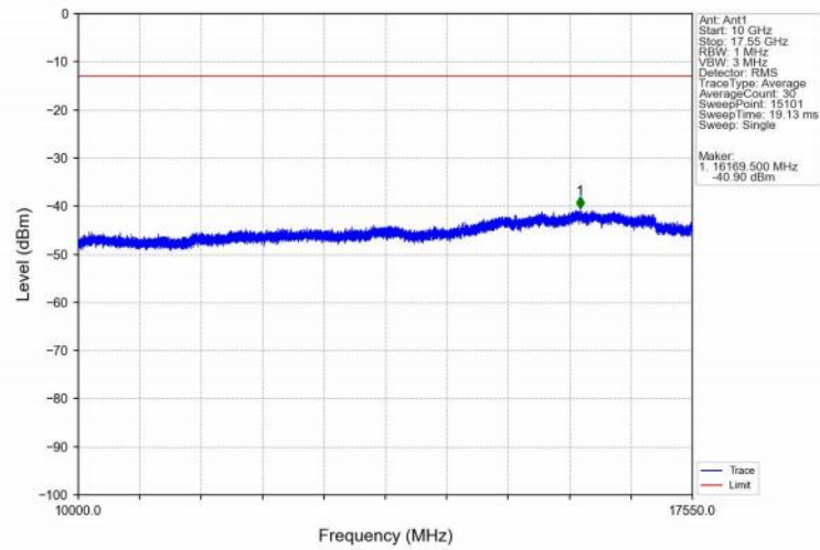
Band4_10MHz_16QAM_MCH_1732.5MHz_RB_1_0_NTNV
