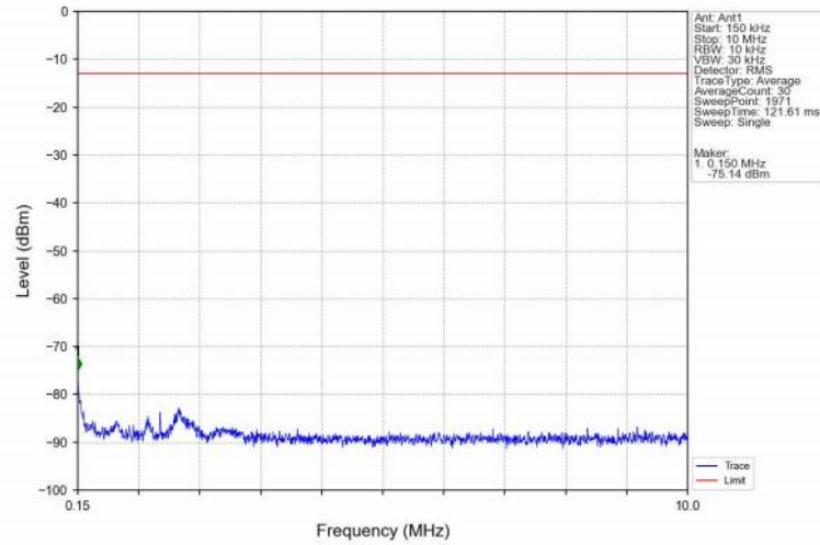
Band4_5MHz_16QAM_HCH_1752.5MHz_RB_1_0_NTNV
