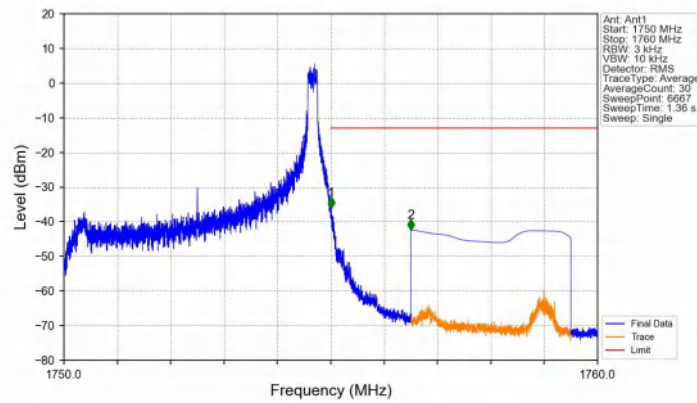
Band4_5MHz_QPSK_HCH_1752.5MHz_RB_1_24_NTNV
