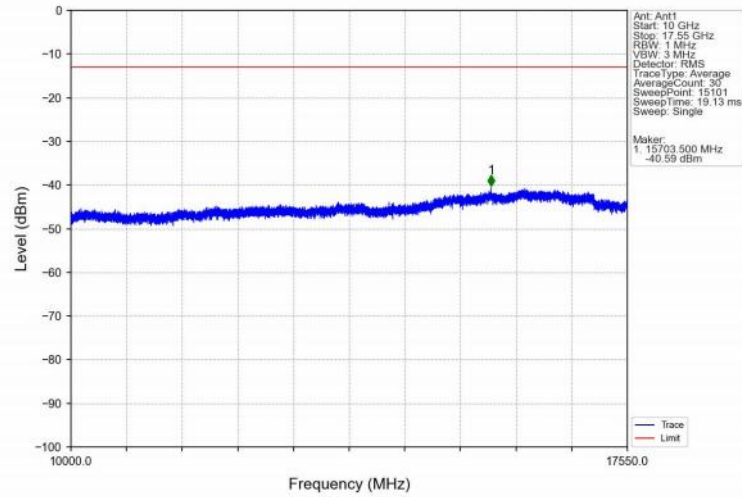
Band4_3MHz_16QAM_LCH_1711.5MHz_RB_15_0_NTNV
