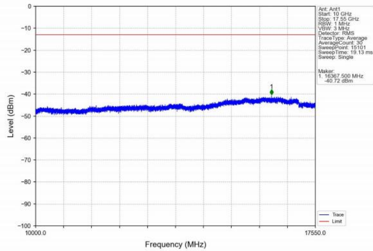
Band4_20MHz_16QAM_HCH_1745MHz_RB_1_99_NTNV
