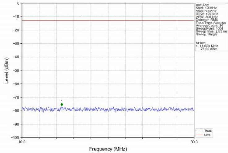
Band4_15MHz_16QAM_HCH_1747.5MHz_RB_1_0_NTNV
