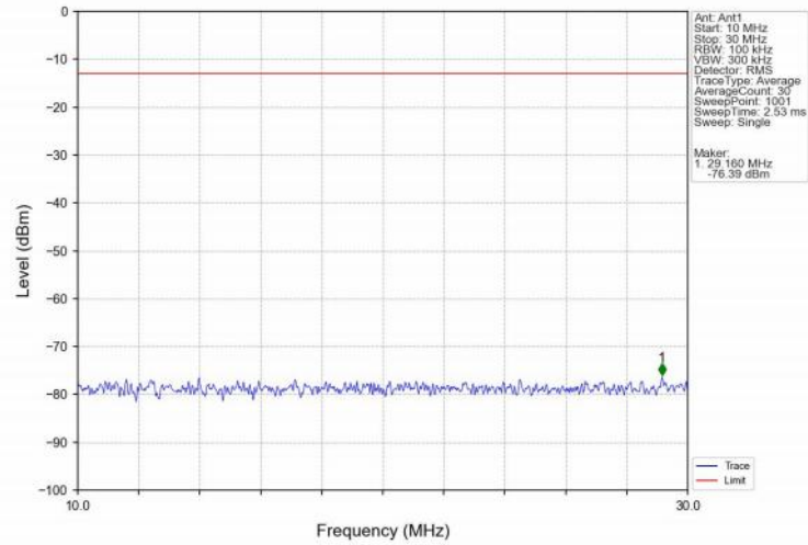
Band4_5MHz_16QAM_MCH_1732.5MHz_RB_1_0_NTNV
