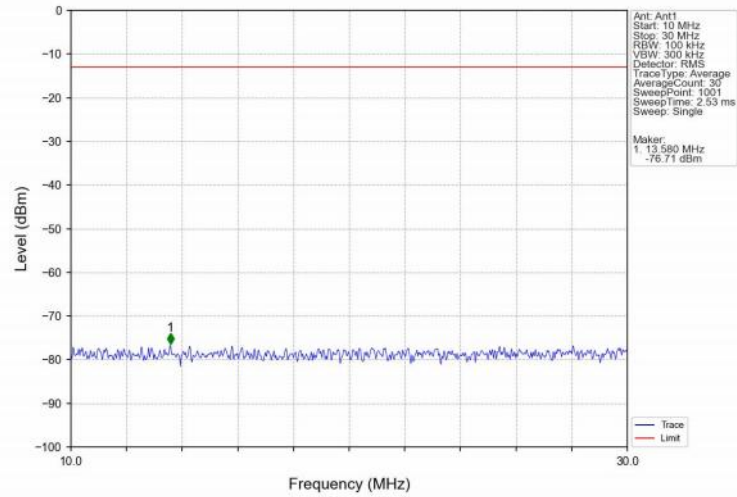
Band4_15MHz_QPSK_HCH_1747.5MHz_RB_1_0_NTNV
