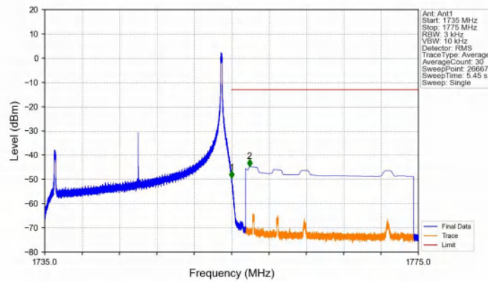
Band4_20MHz_16QAM_HCH_1745MHz_RB_1_99_NTNV
