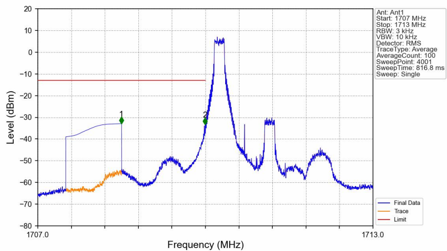
Band4_1.4MHz_16QAM_LCH_1710.7MHz_RB_1_0_NTNV
