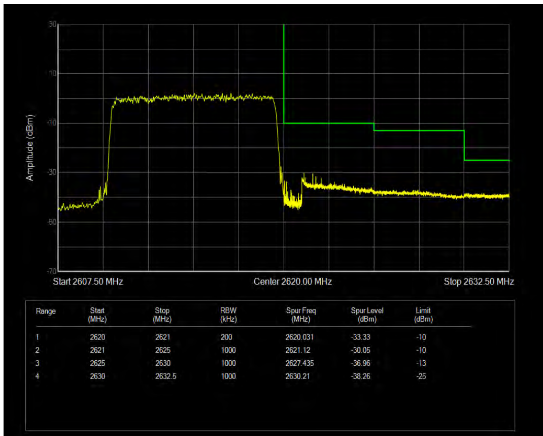
Band38 QAM16 BW=10MHz Channel=38200 RB Size=27 Position=#0
