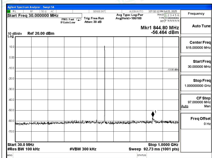
Channel 1 / 560 MHz
