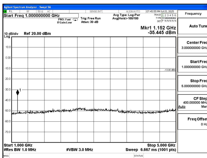
Channel 16 / 575 MHz
