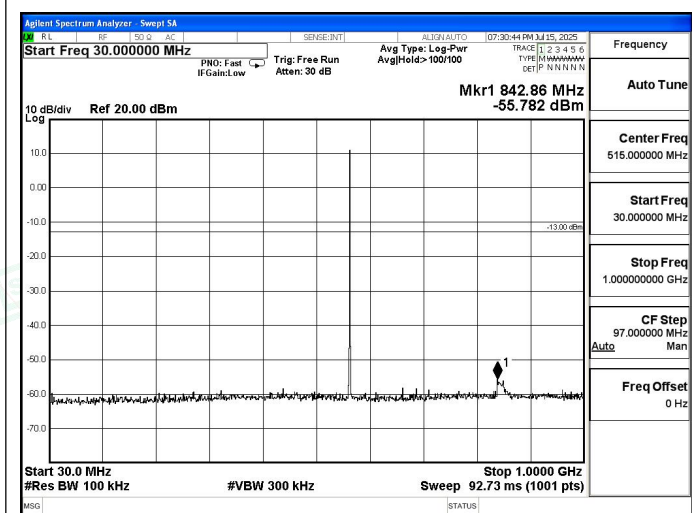
Channel 16 / 575 MHz
