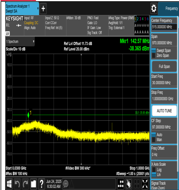
Band41-10MHz-QPSK-40620-1RB#0-30~1000-PASS
