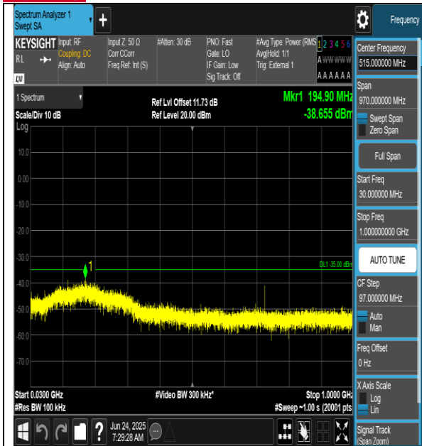
Band41-10MHz-QPSK-41540-1RB#0-30~1000-PASS
