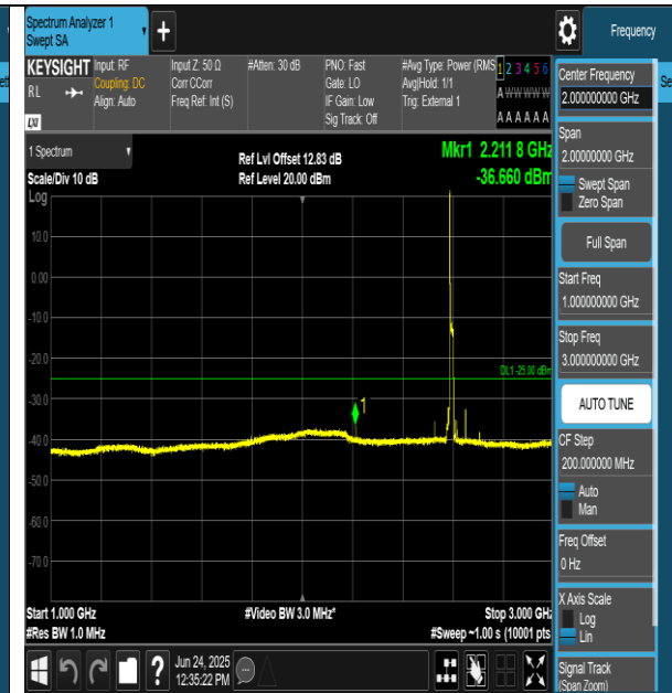
Band41-15MHz-QPSK-40620-1RB#0-1000~3000-PASS
