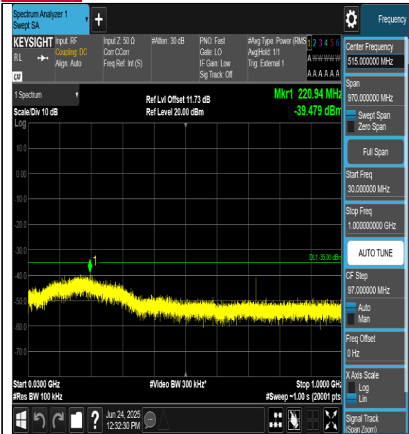
Band41-15MHz-QPSK-39725-1RB#0-30~1000-PASS
