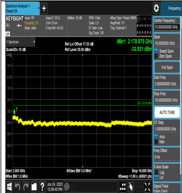
Band41-20MHz-QPSK-39750-1RB#0-3000~18000-PASS
