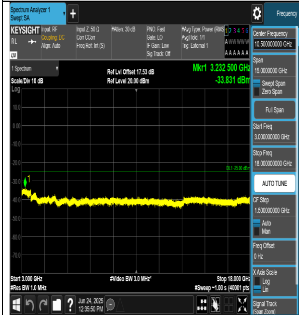
Band41-15MHz-QPSK-40620-1RB#0-3000~18000-PASS
