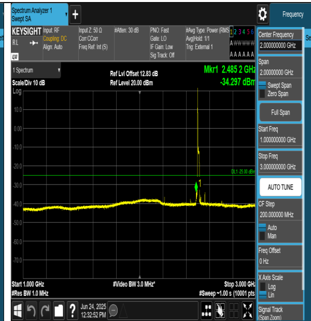
Band41-15MHz-QPSK-39725-1RB#0-1000~3000-PASS
