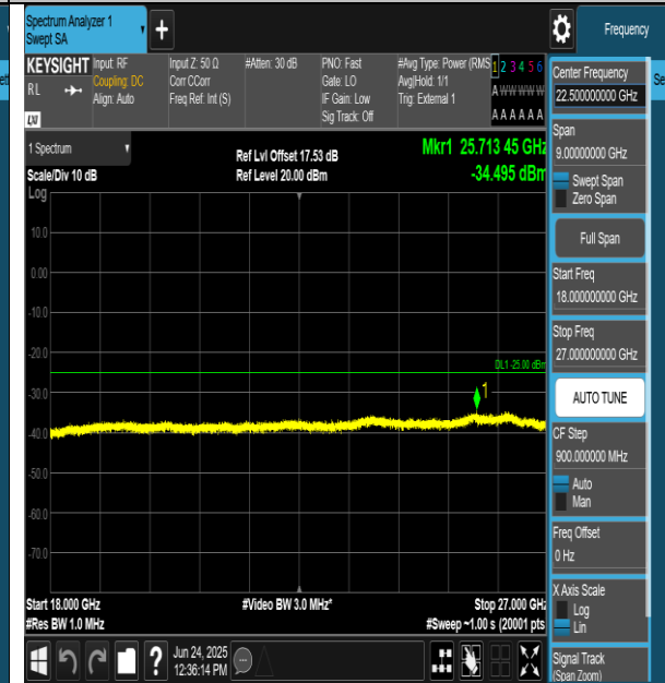
Band41-15MHz-QPSK-40620-1RB#0-18000~27000-PASS
