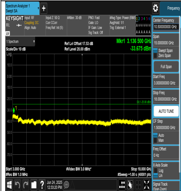
Band41-15MHz-QPSK-39725-1RB#0-3000~18000-PASS
