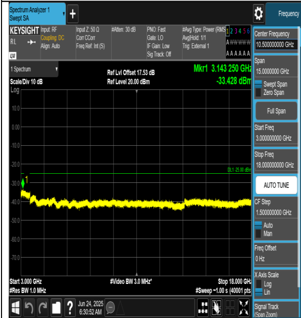
Band41-10MHz-QPSK-40620-1RB#0-3000~18000-PASS
