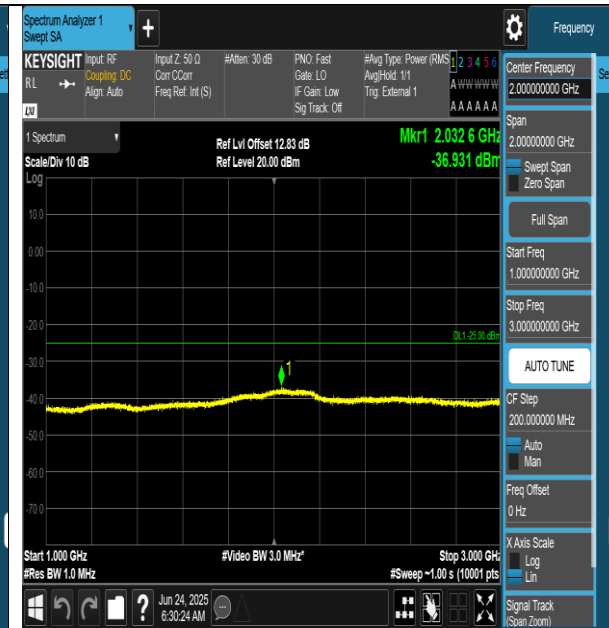
Band41-10MHz-QPSK-40620-1RB#0-1000~3000-PASS
