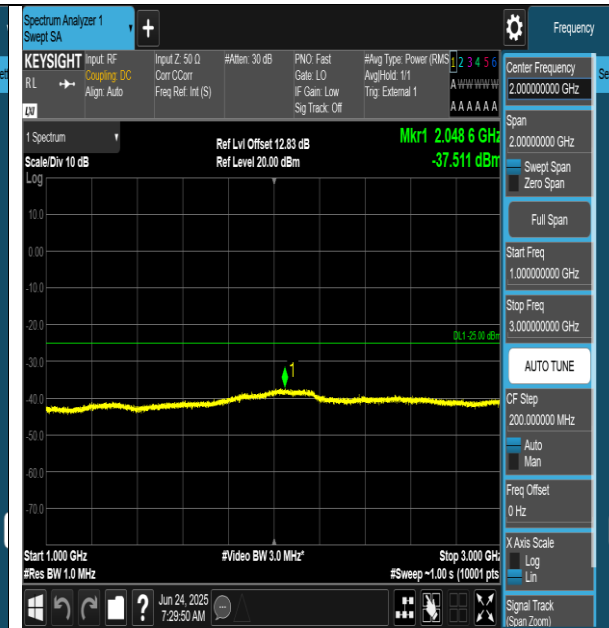
Band41-10MHz-QPSK-41540-1RB#0-1000~3000-PASS
