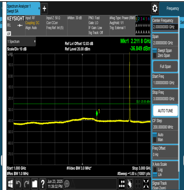
Band41-5MHz-QPSK-41565-1RB#0-1000~3000-PASS
