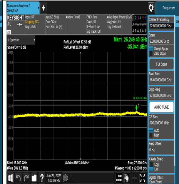
Band41-20MHz-QPSK-39750-1RB#0-18000~27000-PASS
