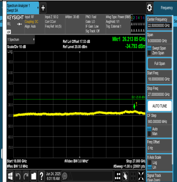
Band41-10MHz-QPSK-40620-1RB#0-18000~27000-PASS
