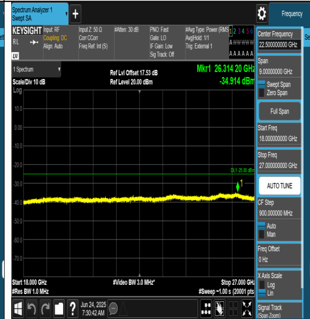
Band41-10MHz-QPSK-41540-1RB#0-18000~27000-PASS
