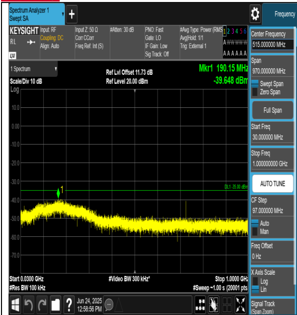
Band41-20MHz-QPSK-39750-1RB#0-30~1000-PASS
