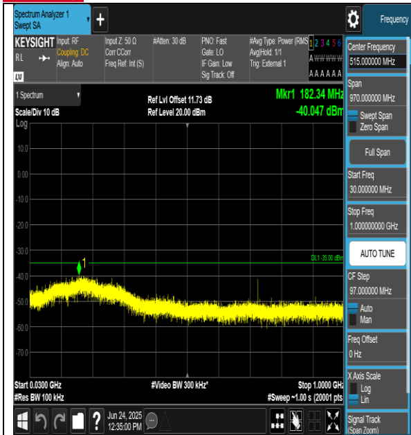
Band41-15MHz-QPSK-40620-1RB#0-30~1000-PASS
