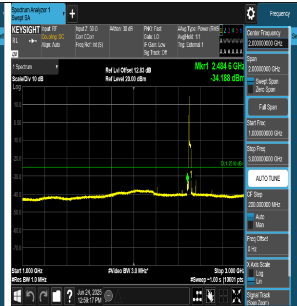
Band41-20MHz-QPSK-39750-1RB#0-1000~3000-PASS
