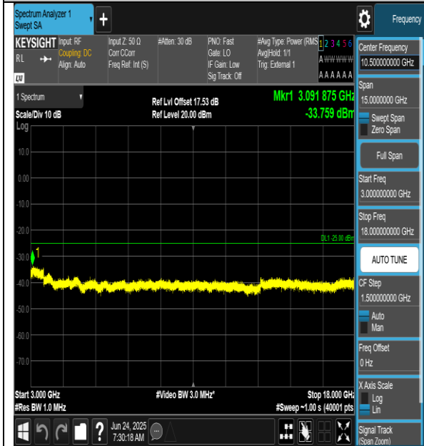
Band41-10MHz-QPSK-41540-1RB#0-3000~18000-PASS
