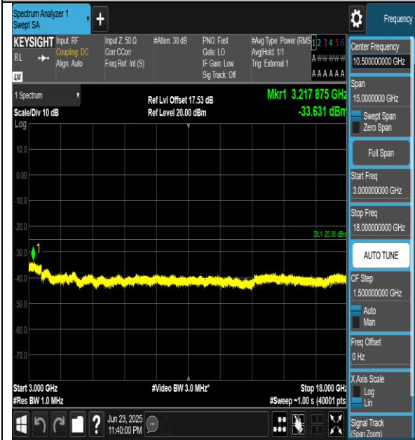
Band41-5MHz-QPSK-41565-1RB#0-3000~18000-PASS
