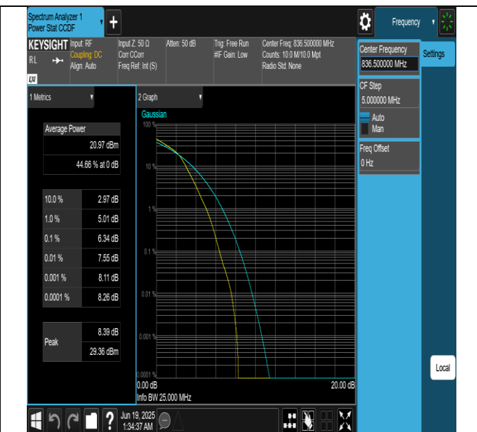
26(824-849)-1.4MHz-16QAM-27033-6RB#0-PASS
